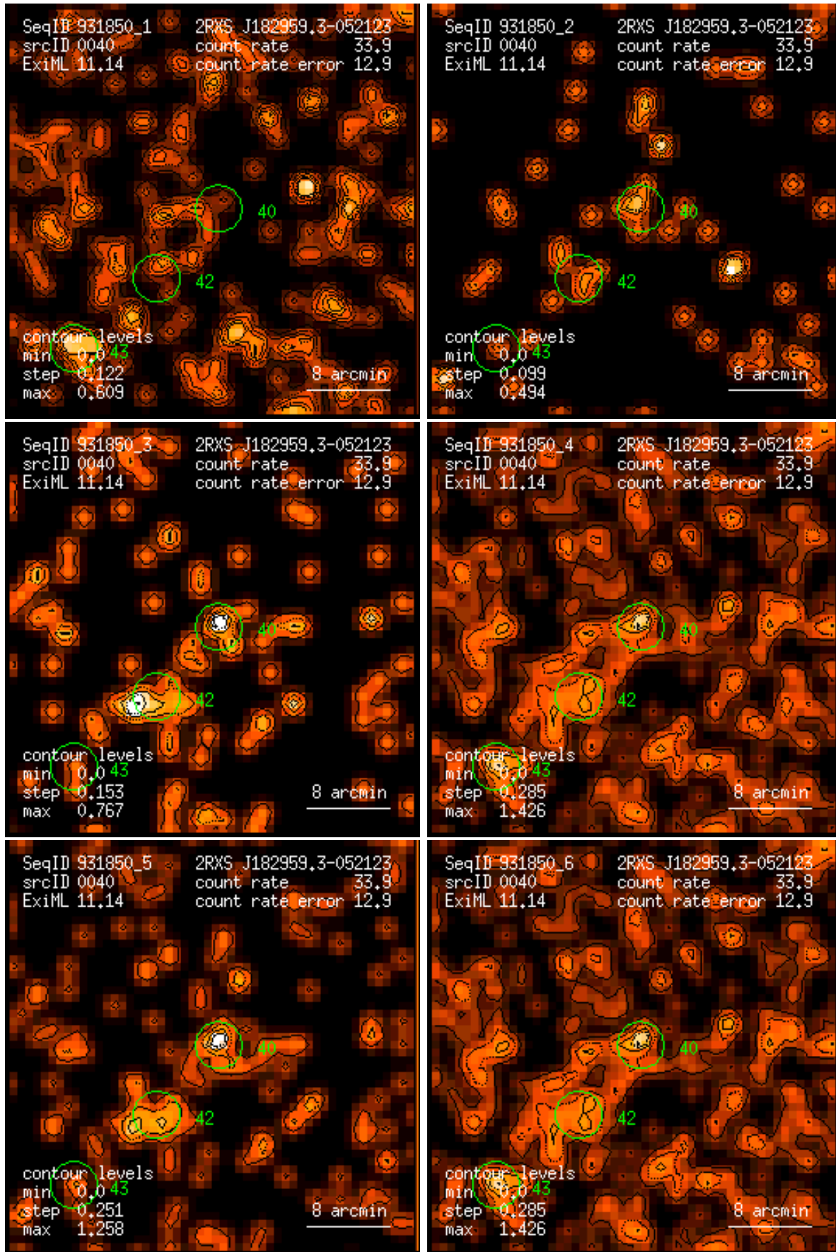
Figure 40: RASS 931850: detection 0040: band rate images, Gaussian filter: (1) PSPC channels 11 – 41, (2) 52 – 90, (3) 91 – 201, (4) 11 – 235, (5) 52 – 201, (6) 11 – 201. Broad band rates in counts/ks. Band rate contour levels in counts/ks/arcmin 2 .
