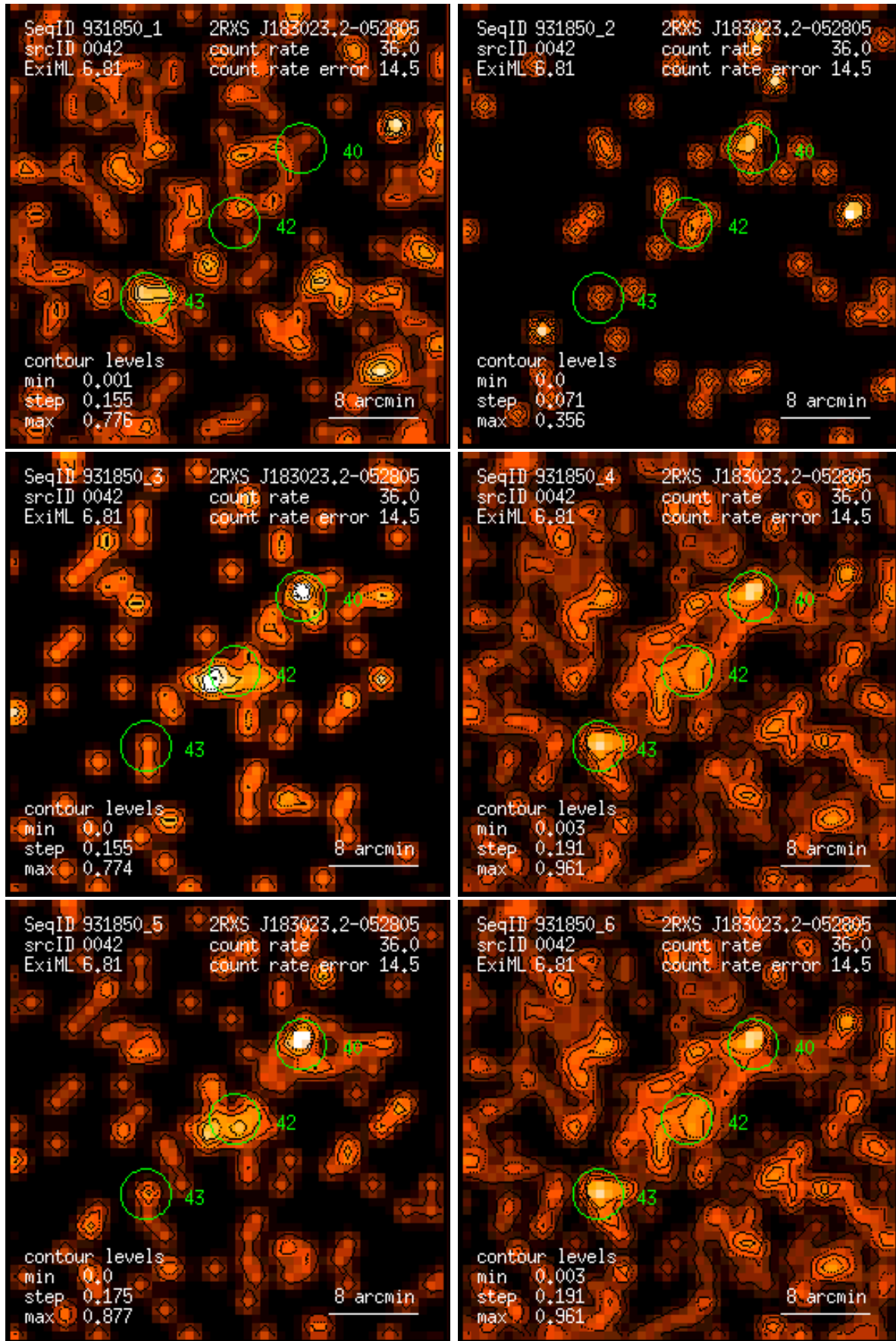
Figure 42: RASS 931850: detection 0042: band rate images, Gaussian filter: (1) PSPC channels 11 – 41, (2) 52 – 90, (3) 91 – 201, (4) 11 – 235, (5) 52 – 201, (6) 11 – 201. Broad band rates in counts/ks. Band rate contour levels in counts/ks/arcmin 2 .
