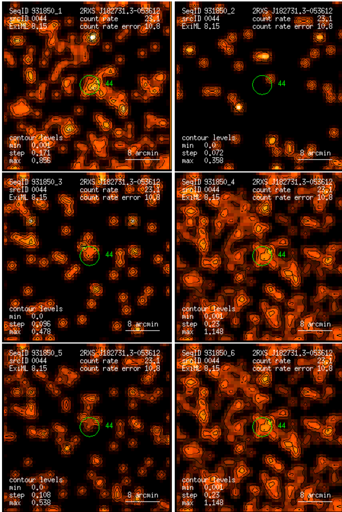
Figure 44: RASS 931850: detection 0044: band rate images, Gaussian filter: (1) PSPC channels 11 – 41, (2) 52 – 90, (3) 91 – 201, (4) 11 – 235, (5) 52 – 201, (6) 11 – 201. Broad band rates in counts/ks. Band rate contour levels in counts/ks/arcmin 2 .
