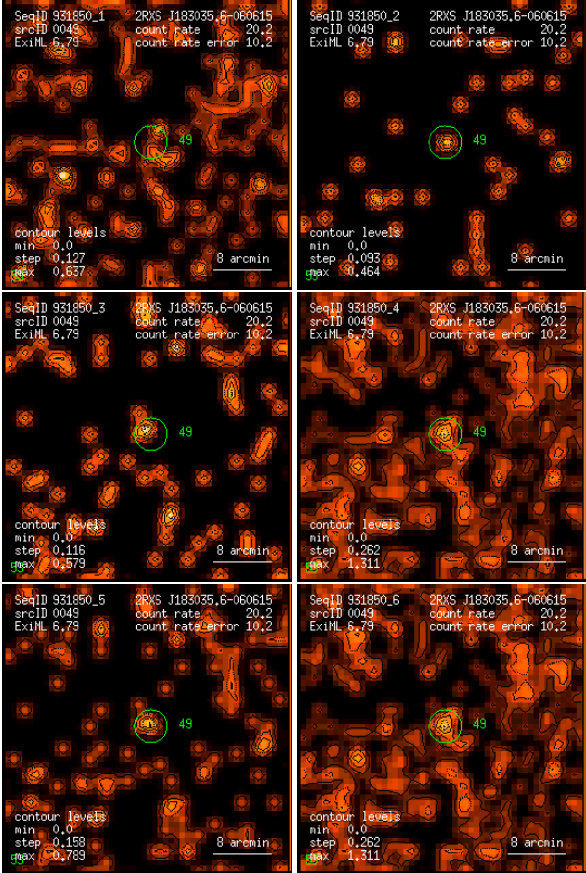
Figure 49: RASS 931850: detection 0049: band rate images, Gaussian filter: (1) PSPC channels 11 – 41, (2) 52 – 90, (3) 91 – 201, (4) 11 – 235, (5) 52 – 201, (6) 11 – 201. Broad band rates in counts/ks. Band rate contour levels in counts/ks/arcmin 2 .
