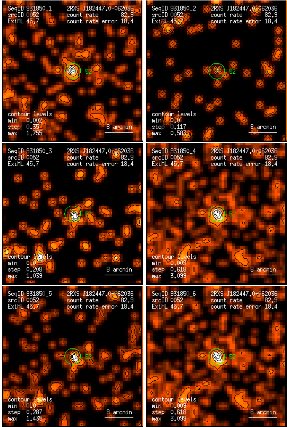
Figure 52: RASS 931850: detection 0052: band rate images, Gaussian filter: (1) PSPC channels 11 – 41, (2) 52 – 90, (3) 91 – 201, (4) 11 – 235, (5) 52 – 201, (6) 11 – 201. Broad band rates in counts/ks. Band rate contour levels in counts/ks/arcmin 2 .
