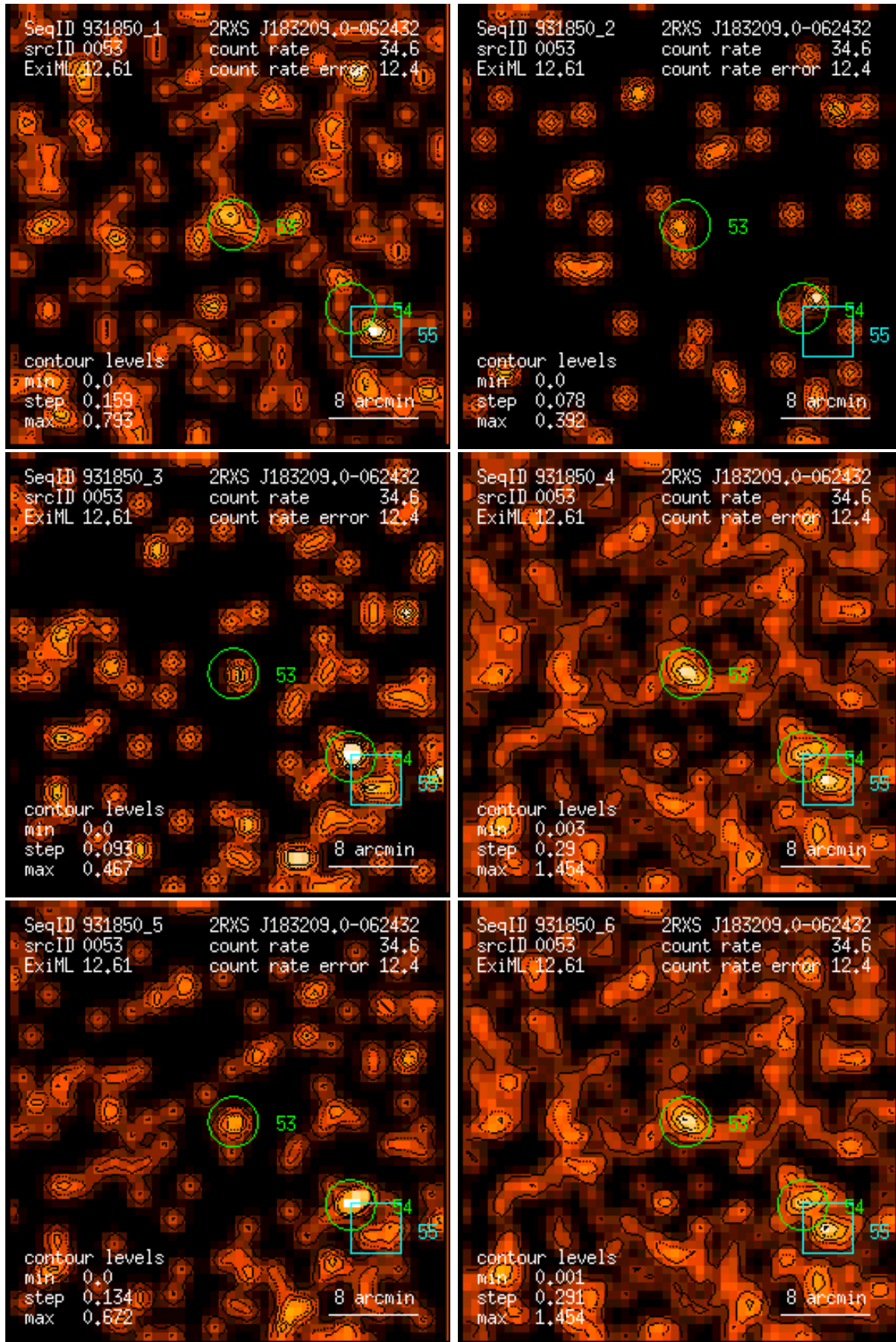
Figure 53: RASS 931850: detection 0053: band rate images, Gaussian filter: (1) PSPC channels 11 – 41, (2) 52 – 90, (3) 91 – 201, (4) 11 – 235, (5) 52 – 201, (6) 11 – 201. Broad band rates in counts/ks. Band rate contour levels in counts/ks/arcmin 2 .
