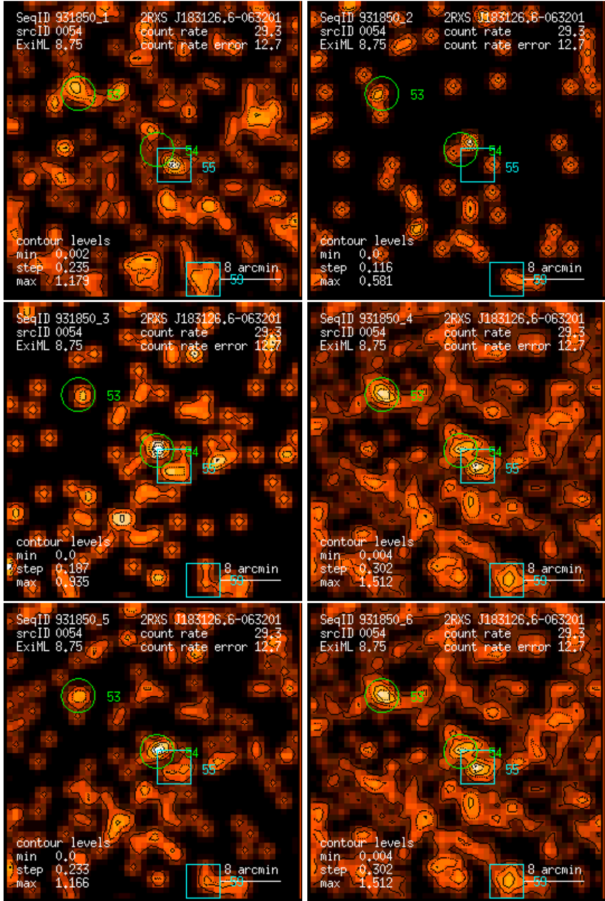
Figure 54: RASS 931850: detection 0054: band rate images, Gaussian filter: (1) PSPC channels 11 – 41, (2) 52 – 90, (3) 91 – 201, (4) 11 – 235, (5) 52 – 201, (6) 11 – 201. Broad band rates in counts/ks. Band rate contour levels in counts/ks/arcmin 2 .
