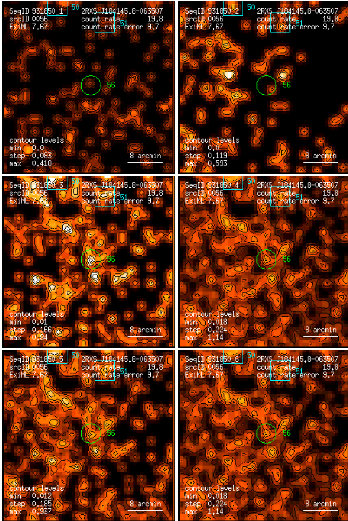
Figure 56: RASS 931850: detection 0056: band rate images, Gaussian filter: (1) PSPC channels 11 – 41, (2) 52 – 90, (3) 91 – 201, (4) 11 – 235, (5) 52 – 201, (6) 11 – 201. Broad band rates in counts/ks. Band rate contour levels in counts/ks/arcmin 2 .
