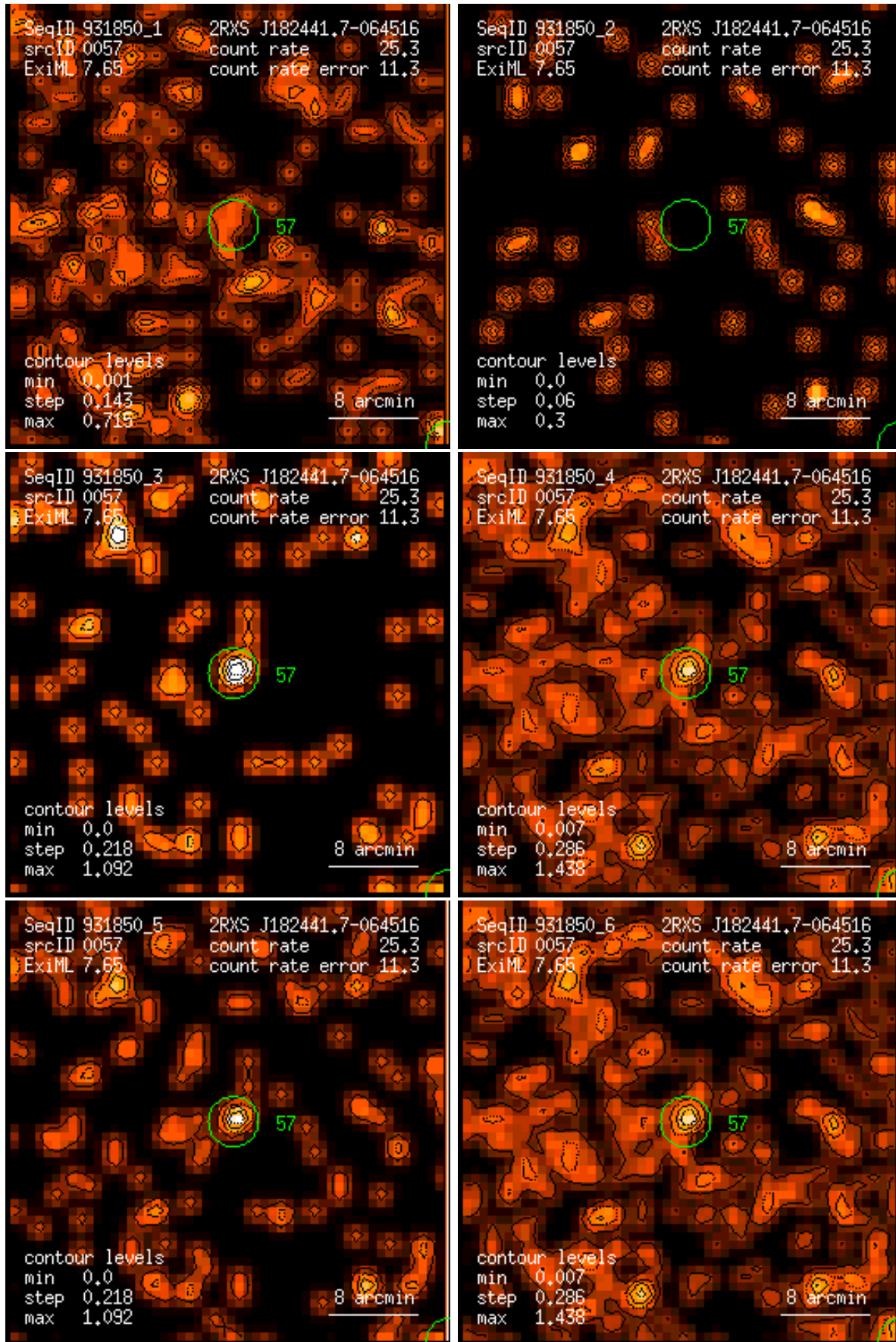
Figure 57: RASS 931850: detection 0057: band rate images, Gaussian filter: (1) PSPC channels 11 – 41, (2) 52 – 90, (3) 91 – 201, (4) 11 – 235, (5) 52 – 201, (6) 11 – 201. Broad band rates in counts/ks. Band rate contour levels in counts/ks/arcmin 2 .
