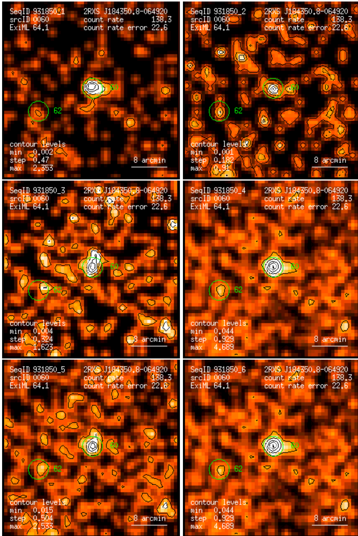
Figure 60: RASS 931850: detection 0060: band rate images, Gaussian filter: (1) PSPC channels 11 – 41, (2) 52 – 90, (3) 91 – 201, (4) 11 – 235, (5) 52 – 201, (6) 11 – 201. Broad band rates in counts/ks. Band rate contour levels in counts/ks/arcmin 2 .
