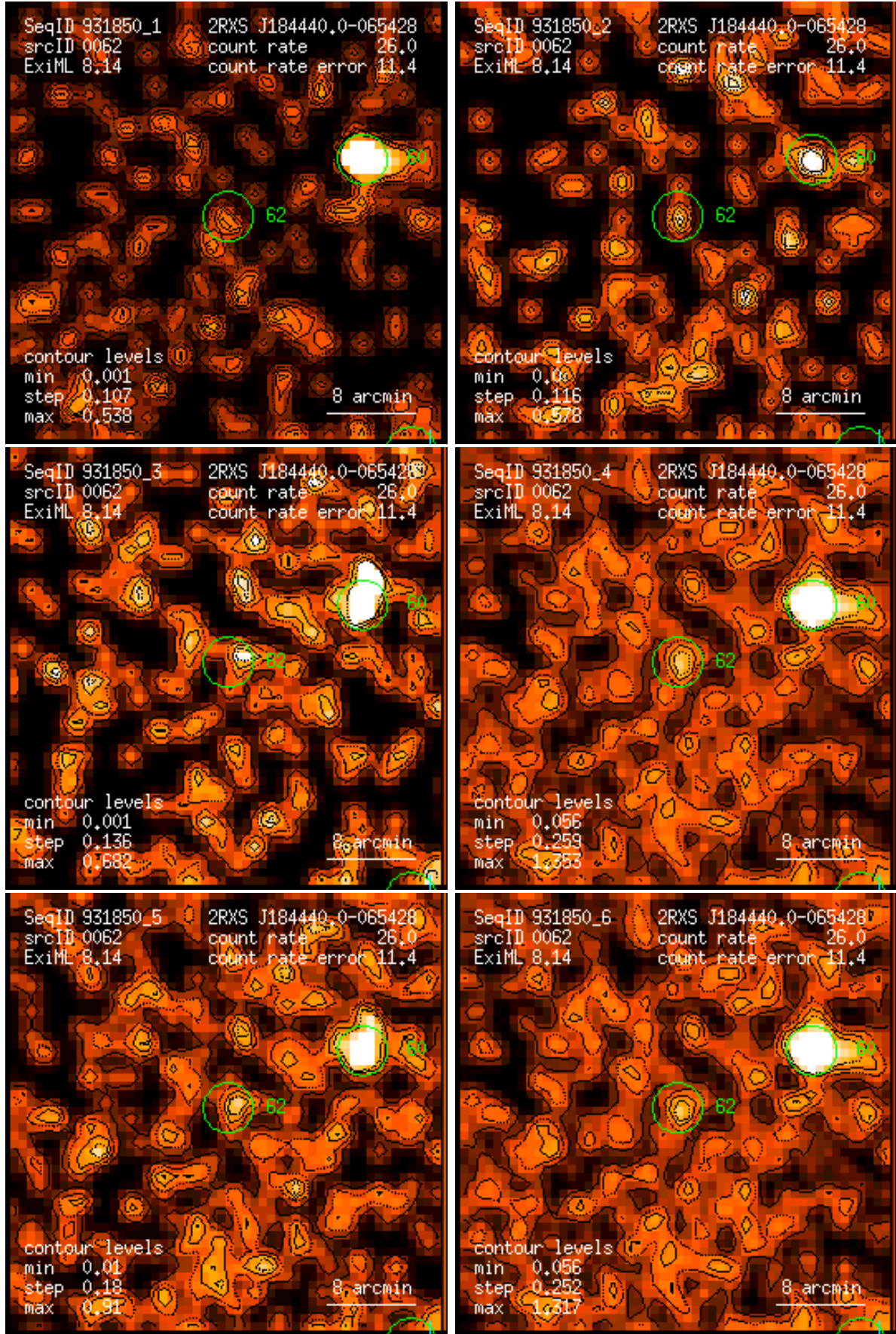
Figure 62: RASS 931850: detection 0062: band rate images, Gaussian filter: (1) PSPC channels 11 – 41, (2) 52 – 90, (3) 91 – 201, (4) 11 – 235, (5) 52 – 201, (6) 11 – 201. Broad band rates in counts/ks. Band rate contour levels in counts/ks/arcmin 2 .
