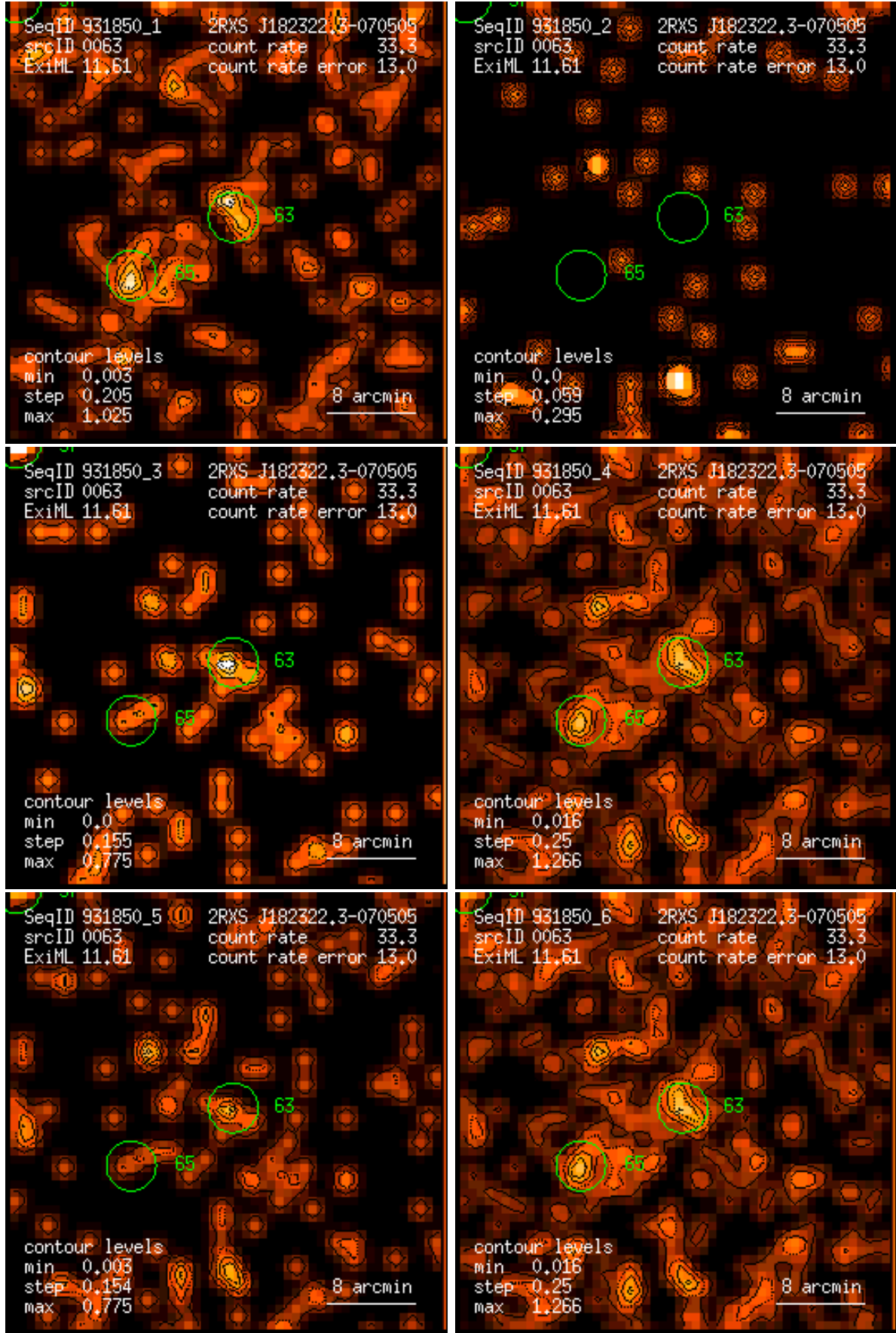
Figure 63: RASS 931850: detection 0063: band rate images, Gaussian filter: (1) PSPC channels 11 – 41, (2) 52 – 90, (3) 91 – 201, (4) 11 – 235, (5) 52 – 201, (6) 11 – 201. Broad band rates in counts/ks. Band rate contour levels in counts/ks/arcmin 2 .
