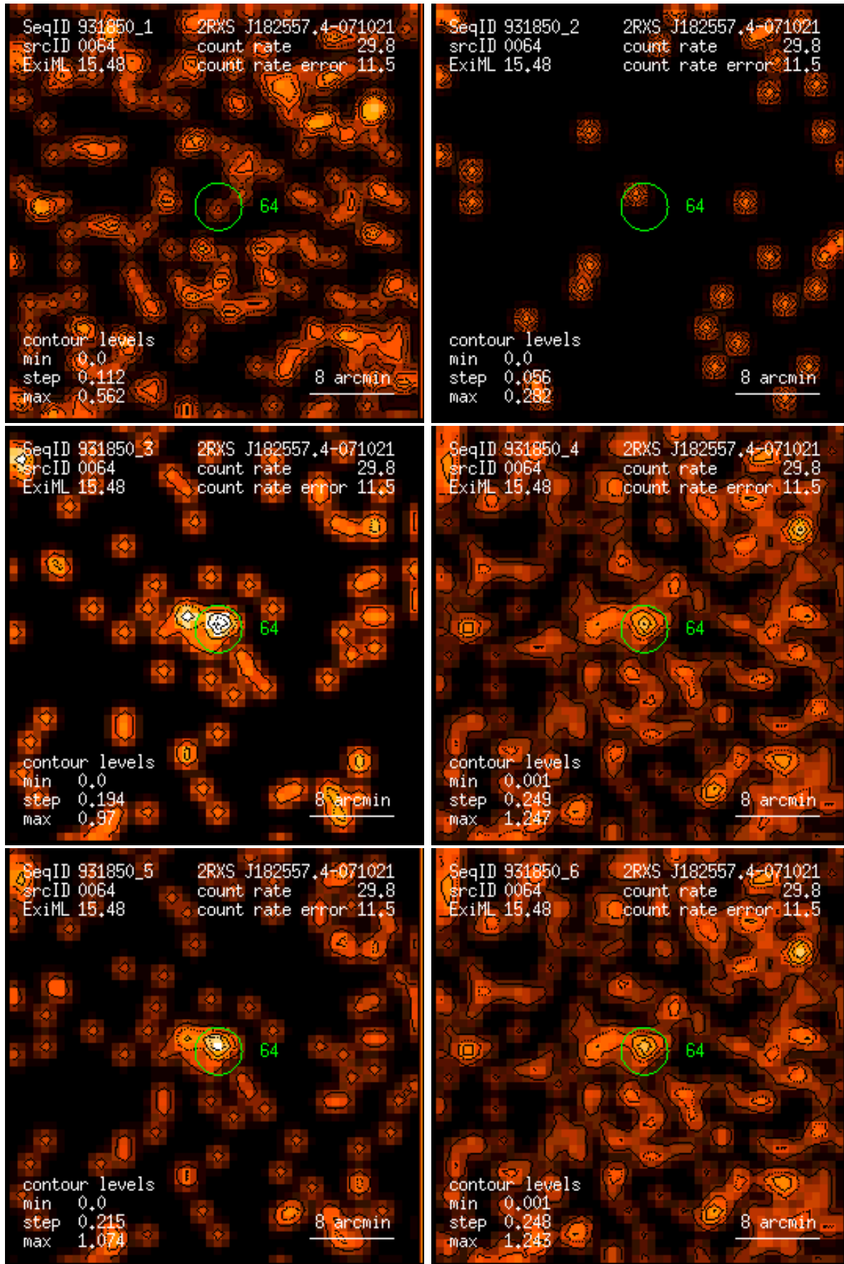
Figure 64: RASS 931850: detection 0064: band rate images, Gaussian filter: (1) PSPC channels 11 – 41, (2) 52 – 90, (3) 91 – 201, (4) 11 – 235, (5) 52 – 201, (6) 11 – 201. Broad band rates in counts/ks. Band rate contour levels in counts/ks/arcmin 2 .
