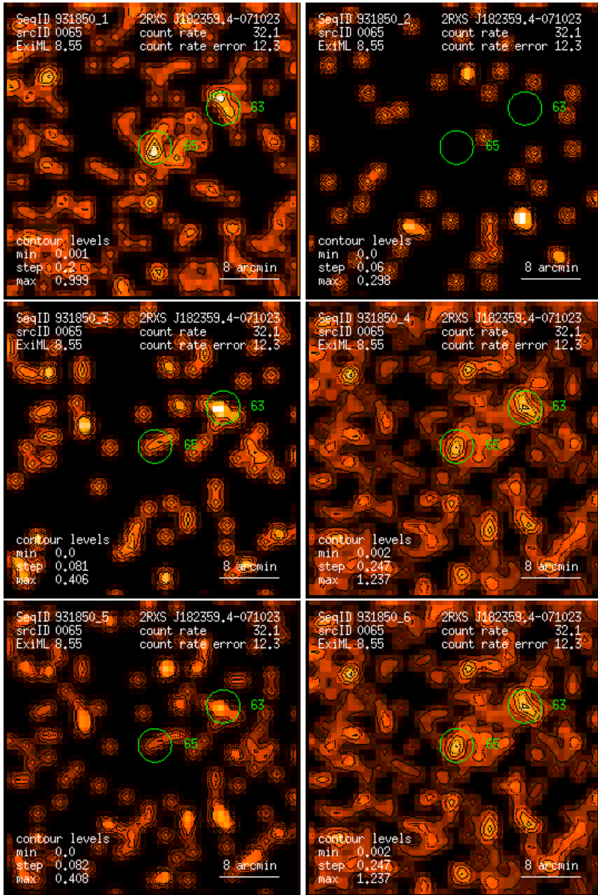
Figure 65: RASS 931850: detection 0065: band rate images, Gaussian filter: (1) PSPC channels 11 – 41, (2) 52 – 90, (3) 91 – 201, (4) 11 – 235, (5) 52 – 201, (6) 11 – 201. Broad band rates in counts/ks. Band rate contour levels in counts/ks/arcmin 2 .
