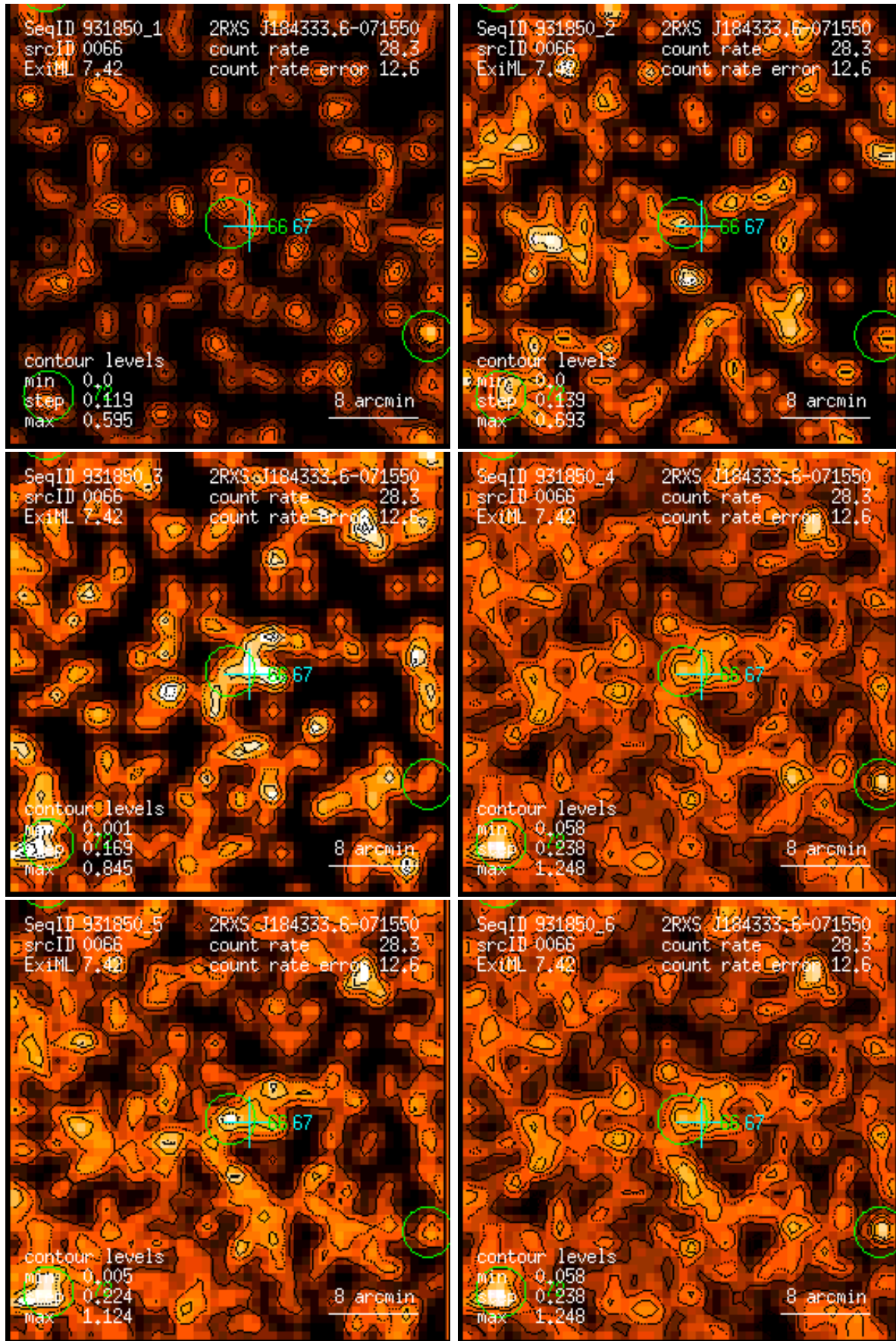
Figure 66: RASS 931850: detection 0066: band rate images, Gaussian filter: (1) PSPC channels 11 – 41, (2) 52 – 90, (3) 91 – 201, (4) 11 – 235, (5) 52 – 201, (6) 11 – 201. Broad band rates in counts/ks. Band rate contour levels in counts/ks/arcmin 2 .
