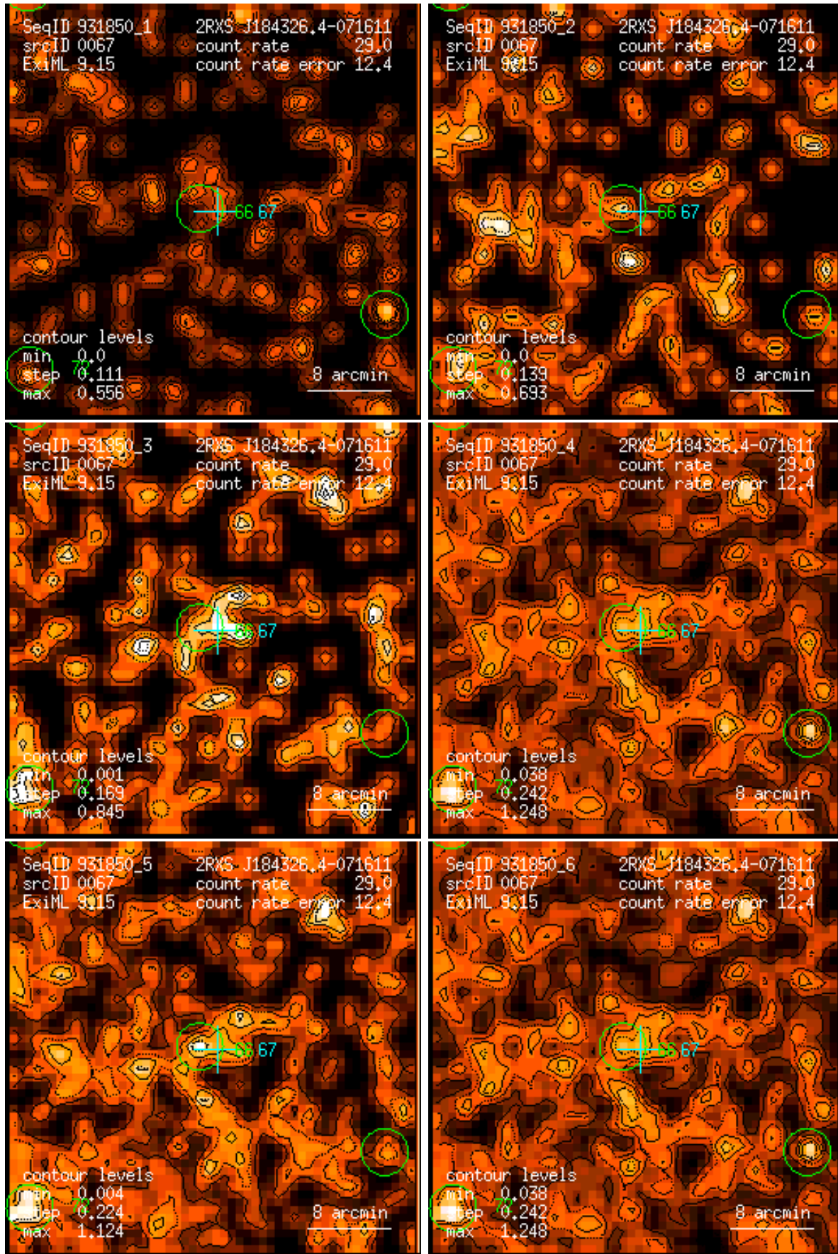
Figure 67: RASS 931850: detection 0067: band rate images, Gaussian filter: (1) PSPC channels 11 – 41, (2) 52 – 90, (3) 91 – 201, (4) 11 – 235, (5) 52 – 201, (6) 11 – 201. Broad band rates in counts/ks. Band rate contour levels in counts/ks/arcmin 2 .
