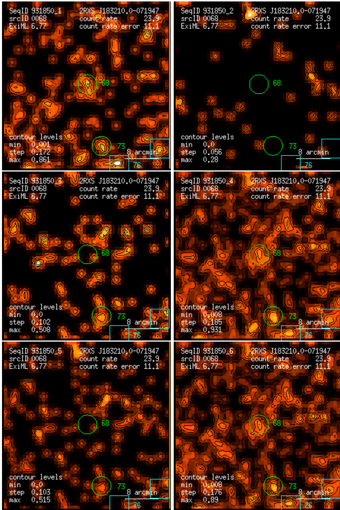
Figure 68: RASS 931850: detection 0068: band rate images, Gaussian filter: (1) PSPC channels 11 – 41, (2) 52 – 90, (3) 91 – 201, (4) 11 – 235, (5) 52 – 201, (6) 11 – 201. Broad band rates in counts/ks. Band rate contour levels in counts/ks/arcmin 2 .
