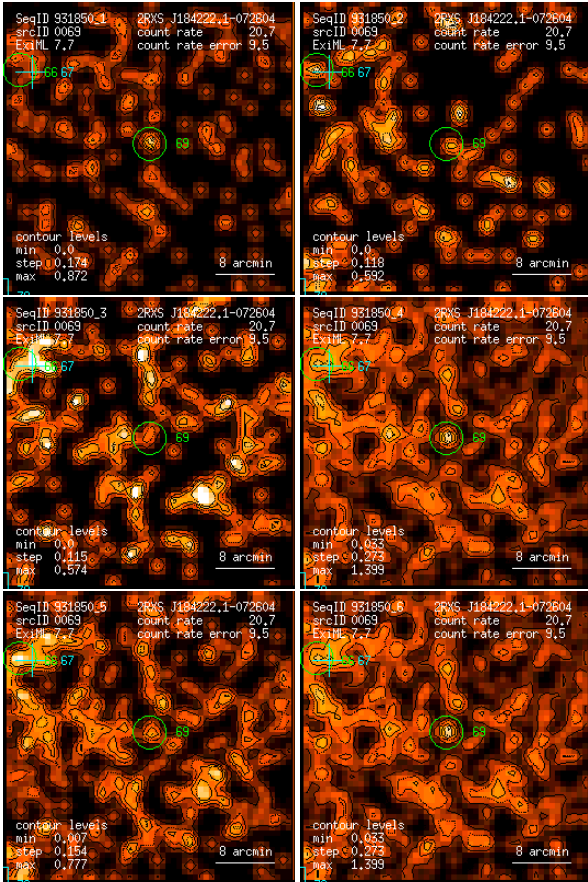
Figure 69: RASS 931850: detection 0069: band rate images, Gaussian filter: (1) PSPC channels 11 – 41, (2) 52 – 90, (3) 91 – 201, (4) 11 – 235, (5) 52 – 201, (6) 11 – 201. Broad band rates in counts/ks. Band rate contour levels in counts/ks/arcmin 2 .
