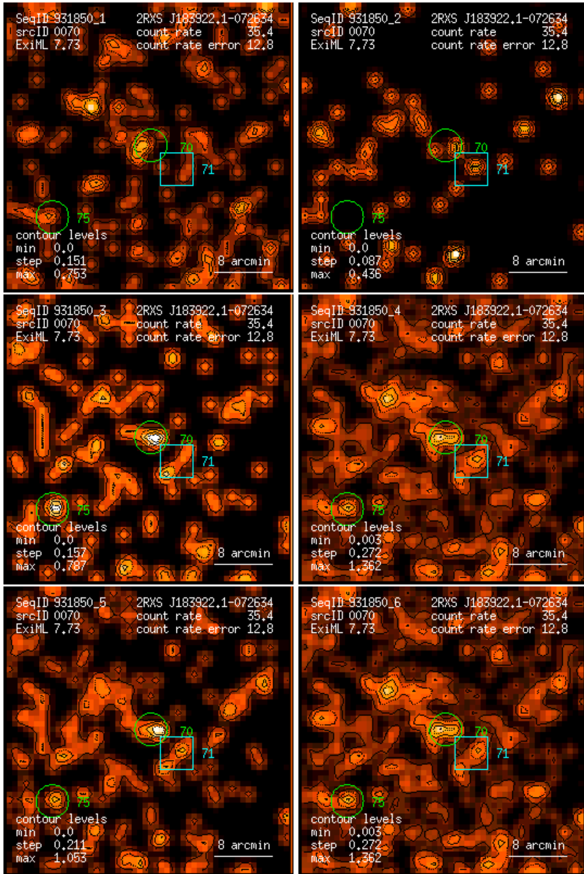
Figure 70: RASS 931850: detection 0070: band rate images, Gaussian filter: (1) PSPC channels 11 – 41, (2) 52 – 90, (3) 91 – 201, (4) 11 – 235, (5) 52 – 201, (6) 11 – 201. Broad band rates in counts/ks. Band rate contour levels in counts/ks/arcmin 2 .
