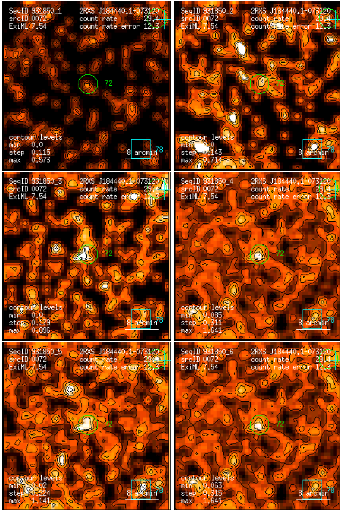
Figure 72: RASS 931850: detection 0072: band rate images, Gaussian filter: (1) PSPC channels 11 – 41, (2) 52 – 90, (3) 91 – 201, (4) 11 – 235, (5) 52 – 201, (6) 11 – 201. Broad band rates in counts/ks. Band rate contour levels in counts/ks/arcmin 2 .
