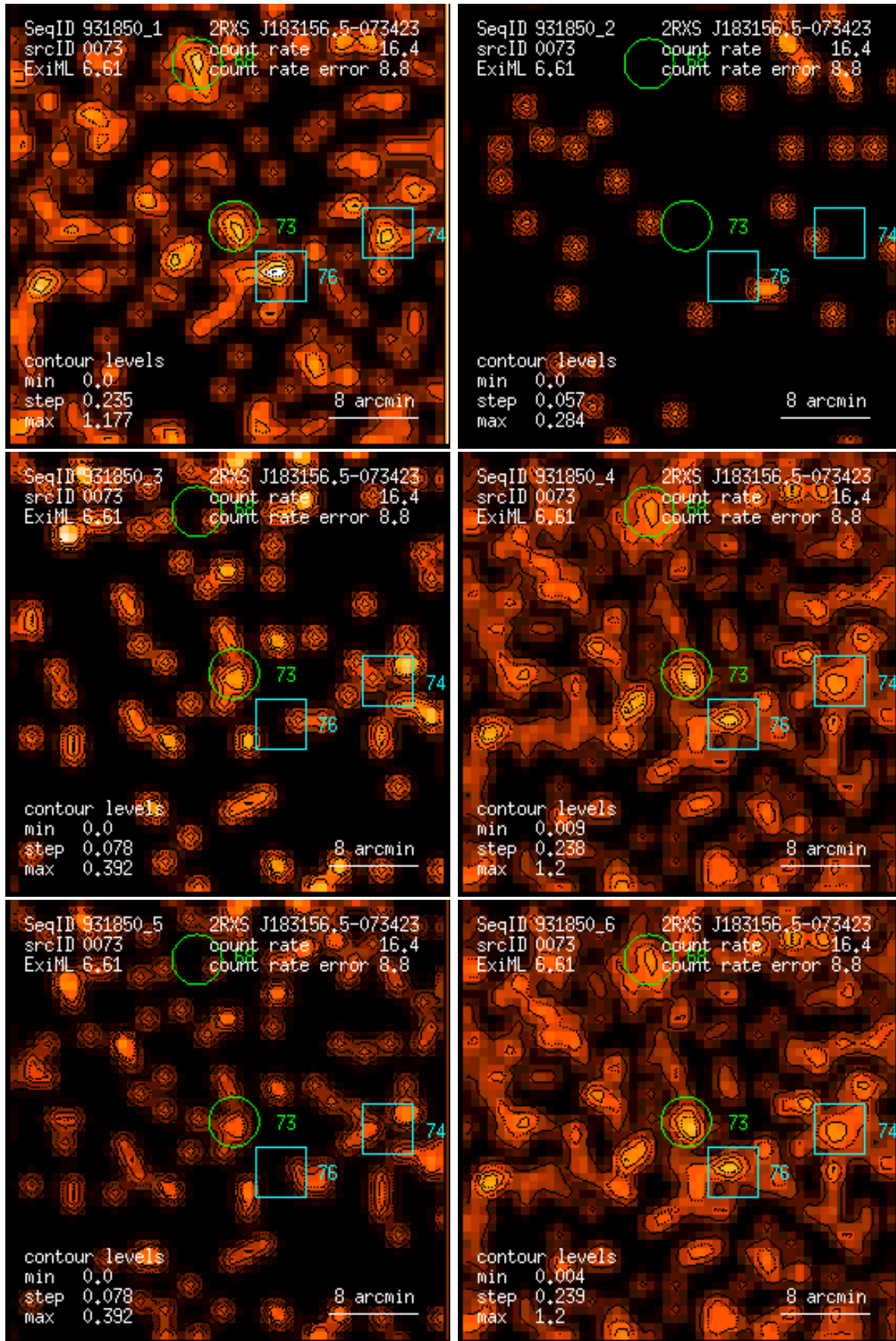
Figure 73: RASS 931850: detection 0073: band rate images, Gaussian filter: (1) PSPC channels 11 – 41, (2) 52 – 90, (3) 91 – 201, (4) 11 – 235, (5) 52 – 201, (6) 11 – 201. Broad band rates in counts/ks. Band rate contour levels in counts/ks/arcmin 2 .
