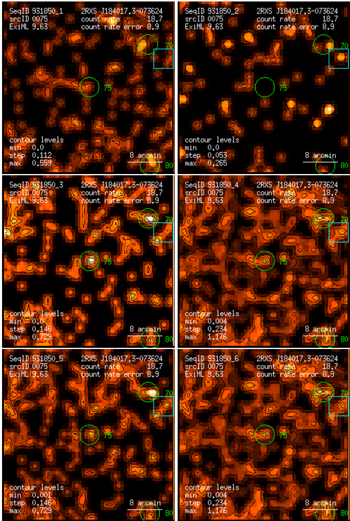
Figure 75: RASS 931850: detection 0075: band rate images, Gaussian filter: (1) PSPC channels 11 – 41, (2) 52 – 90, (3) 91 – 201, (4) 11 – 235, (5) 52 – 201, (6) 11 – 201. Broad band rates in counts/ks. Band rate contour levels in counts/ks/arcmin 2 .
