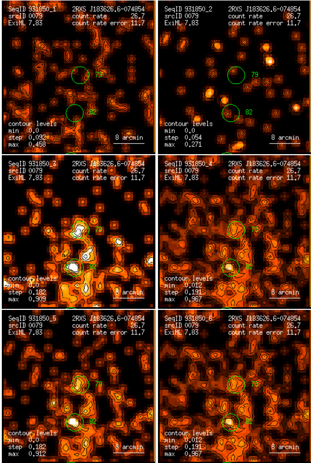
Figure 79: RASS 931850: detection 0079: band rate images, Gaussian filter: (1) PSPC channels 11 – 41, (2) 52 – 90, (3) 91 – 201, (4) 11 – 235, (5) 52 – 201, (6) 11 – 201. Broad band rates in counts/ks. Band rate contour levels in counts/ks/arcmin 2 .
