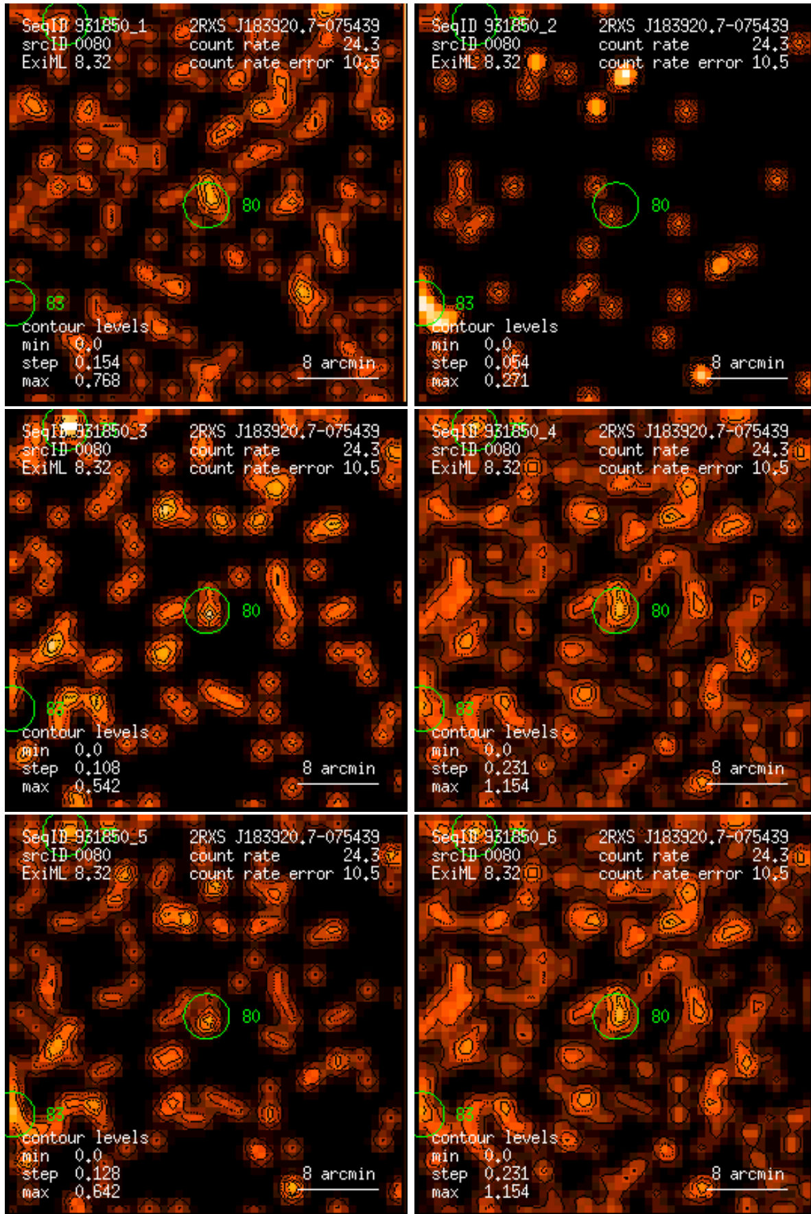
Figure 80: RASS 931850: detection 0080: band rate images, Gaussian filter: (1) PSPC channels 11 – 41, (2) 52 – 90, (3) 91 – 201, (4) 11 – 235, (5) 52 – 201, (6) 11 – 201. Broad band rates in counts/ks. Band rate contour levels in counts/ks/arcmin 2 .
