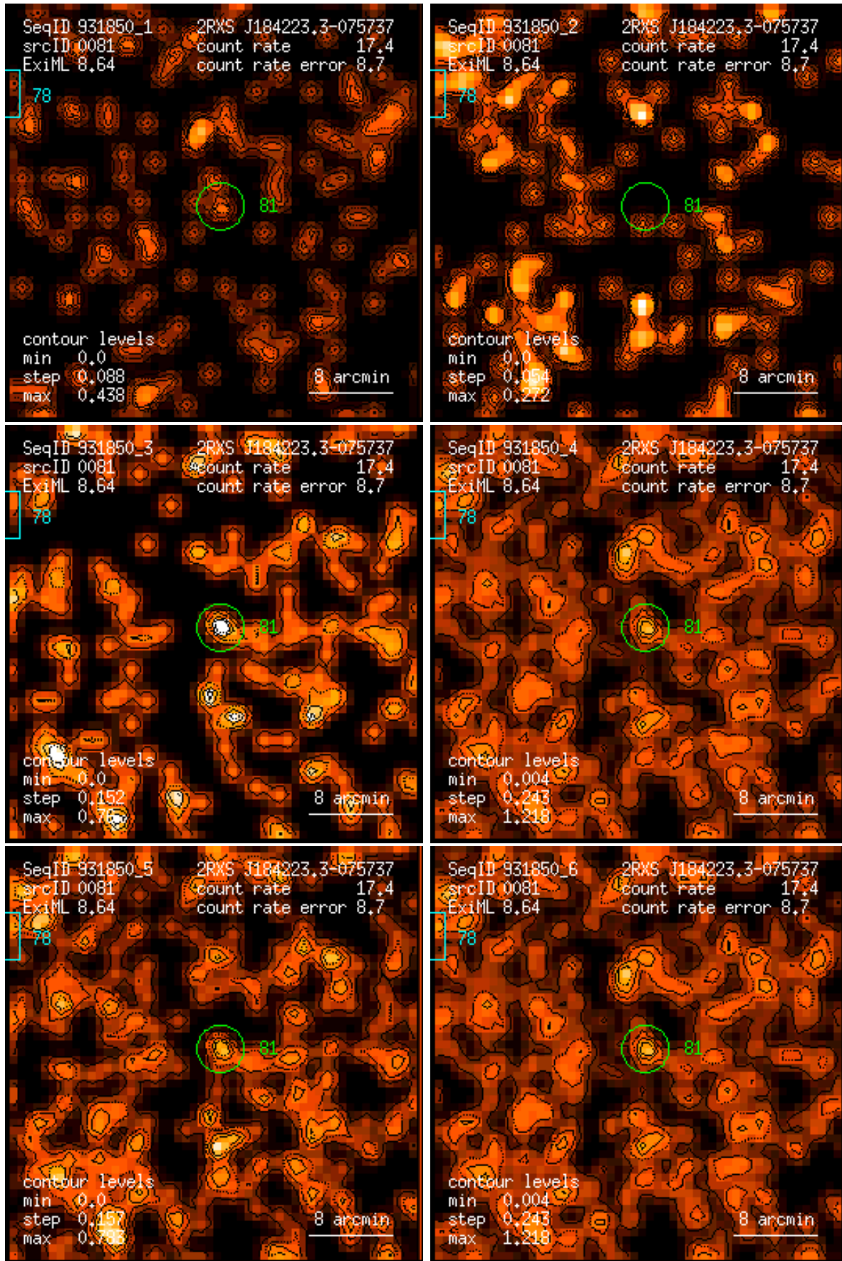
Figure 81: RASS 931850: detection 0081: band rate images, Gaussian filter: (1) PSPC channels 11 – 41, (2) 52 – 90, (3) 91 – 201, (4) 11 – 235, (5) 52 – 201, (6) 11 – 201. Broad band rates in counts/ks. Band rate contour levels in counts/ks/arcmin 2 .
