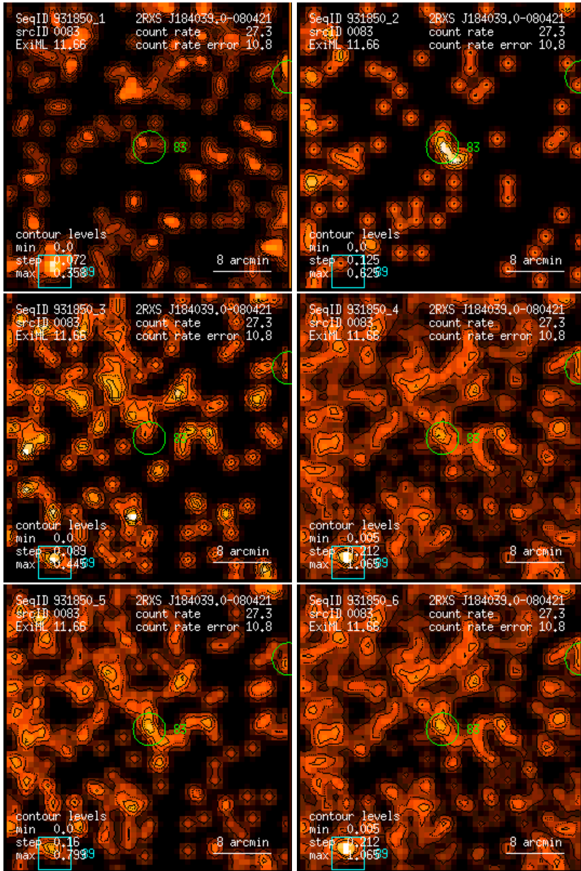
Figure 83: RASS 931850: detection 0083: band rate images, Gaussian filter: (1) PSPC channels 11 – 41, (2) 52 – 90, (3) 91 – 201, (4) 11 – 235, (5) 52 – 201, (6) 11 – 201. Broad band rates in counts/ks. Band rate contour levels in counts/ks/arcmin 2 .
