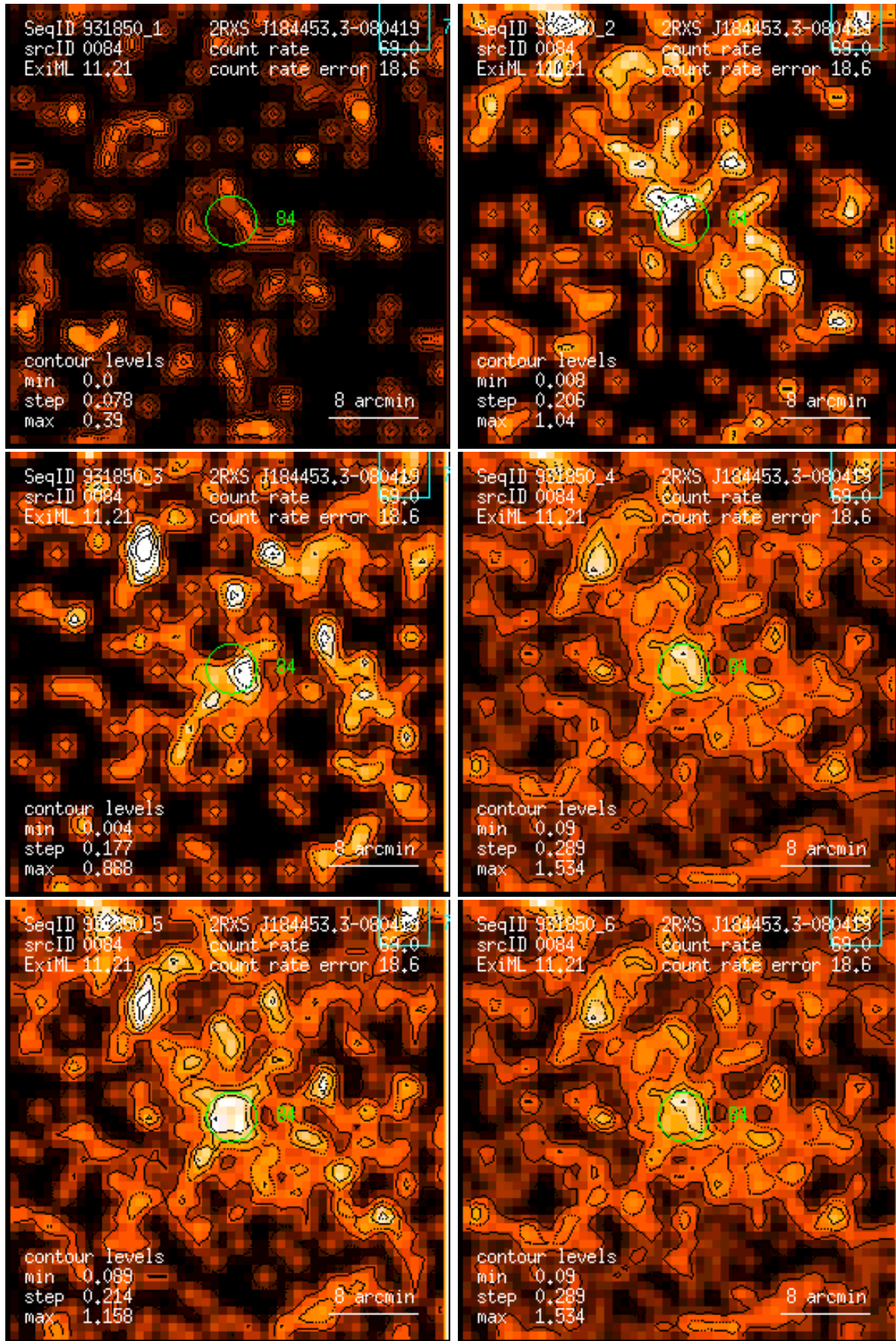
Figure 84: RASS 931850: detection 0084: band rate images, Gaussian filter: (1) PSPC channels 11 – 41, (2) 52 – 90, (3) 91 – 201, (4) 11 – 235, (5) 52 – 201, (6) 11 – 201. Broad band rates in counts/ks. Band rate contour levels in counts/ks/arcmin 2 .
