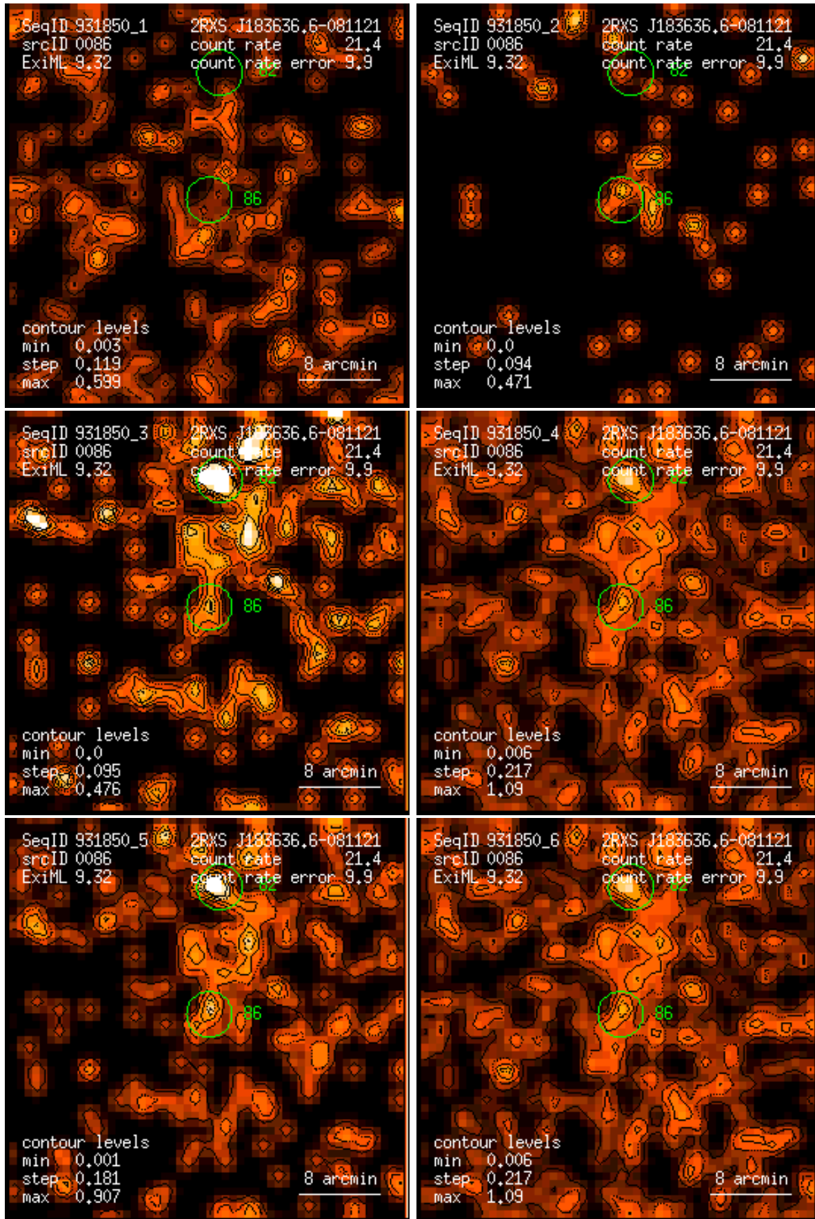
Figure 86: RASS 931850: detection 0086: band rate images, Gaussian filter: (1) PSPC channels 11 – 41, (2) 52 – 90, (3) 91 – 201, (4) 11 – 235, (5) 52 – 201, (6) 11 – 201. Broad band rates in counts/ks. Band rate contour levels in counts/ks/arcmin 2 .
