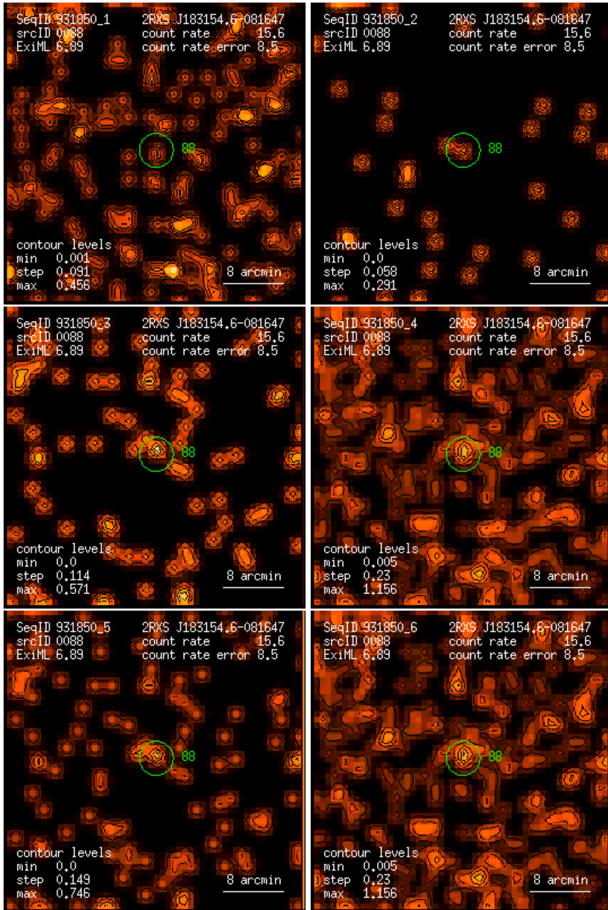
Figure 88: RASS 931850: detection 0088: band rate images, Gaussian filter: (1) PSPC channels 11 – 41, (2) 52 – 90, (3) 91 – 201, (4) 11 – 235, (5) 52 – 201, (6) 11 – 201. Broad band rates in counts/ks. Band rate contour levels in counts/ks/arcmin 2 .
