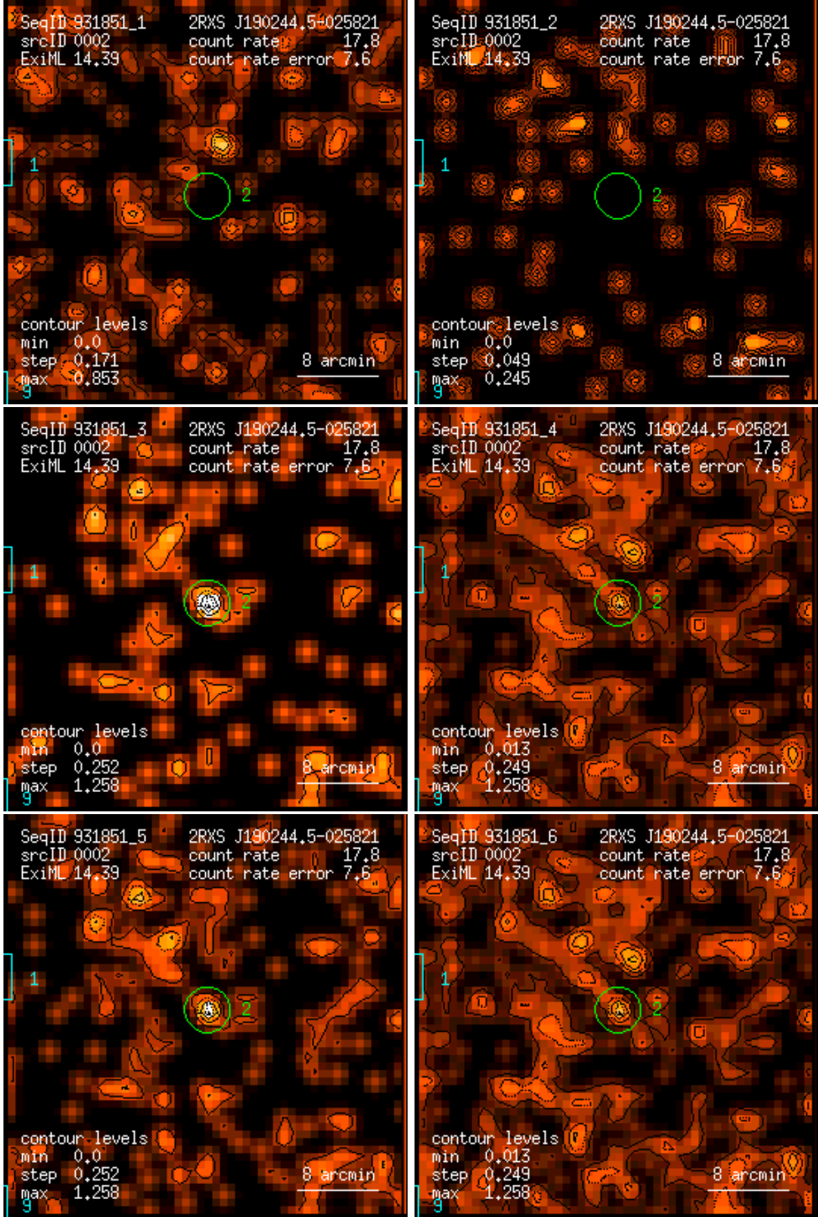
Figure 2: RASS 931851: detection 0002: band rate images, Gaussian filter: (1) PSPC channels 11 – 41, (2) 52 – 90, (3) 91 – 201, (4) 11 – 235, (5) 52 – 201, (6) 11 – 201. Broad band rates in counts/ks. Band rate contour levels in counts/ks/arcmin 2 .
