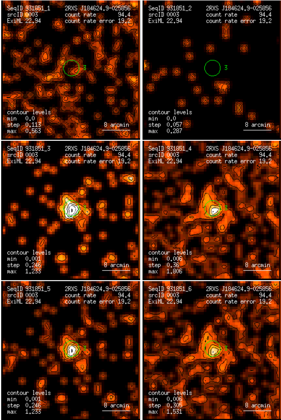
Figure 3: RASS 931851: detection 0003: band rate images, Gaussian filter: (1) PSPC channels 11 – 41, (2) 52 – 90, (3) 91 – 201, (4) 11 – 235, (5) 52 – 201, (6) 11 – 201. Broad band rates in counts/ks. Band rate contour levels in counts/ks/arcmin 2 .
