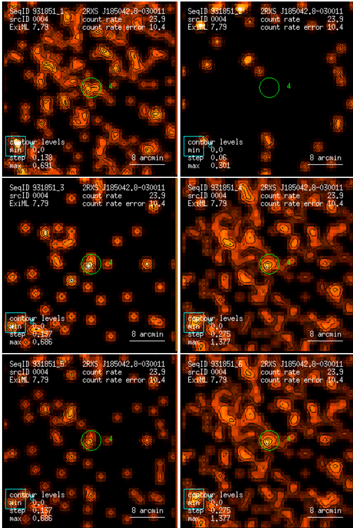
Figure 4: RASS 931851: detection 0004: band rate images, Gaussian filter: (1) PSPC channels 11 – 41, (2) 52 – 90, (3) 91 – 201, (4) 11 – 235, (5) 52 – 201, (6) 11 – 201. Broad band rates in counts/ks. Band rate contour levels in counts/ks/arcmin 2 .
