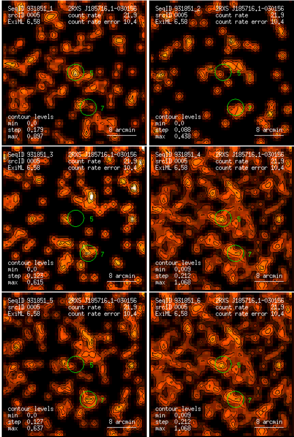
Figure 5: RASS 931851: detection 0005: band rate images, Gaussian filter: (1) PSPC channels 11 – 41, (2) 52 – 90, (3) 91 – 201, (4) 11 – 235, (5) 52 – 201, (6) 11 – 201. Broad band rates in counts/ks. Band rate contour levels in counts/ks/arcmin 2 .
