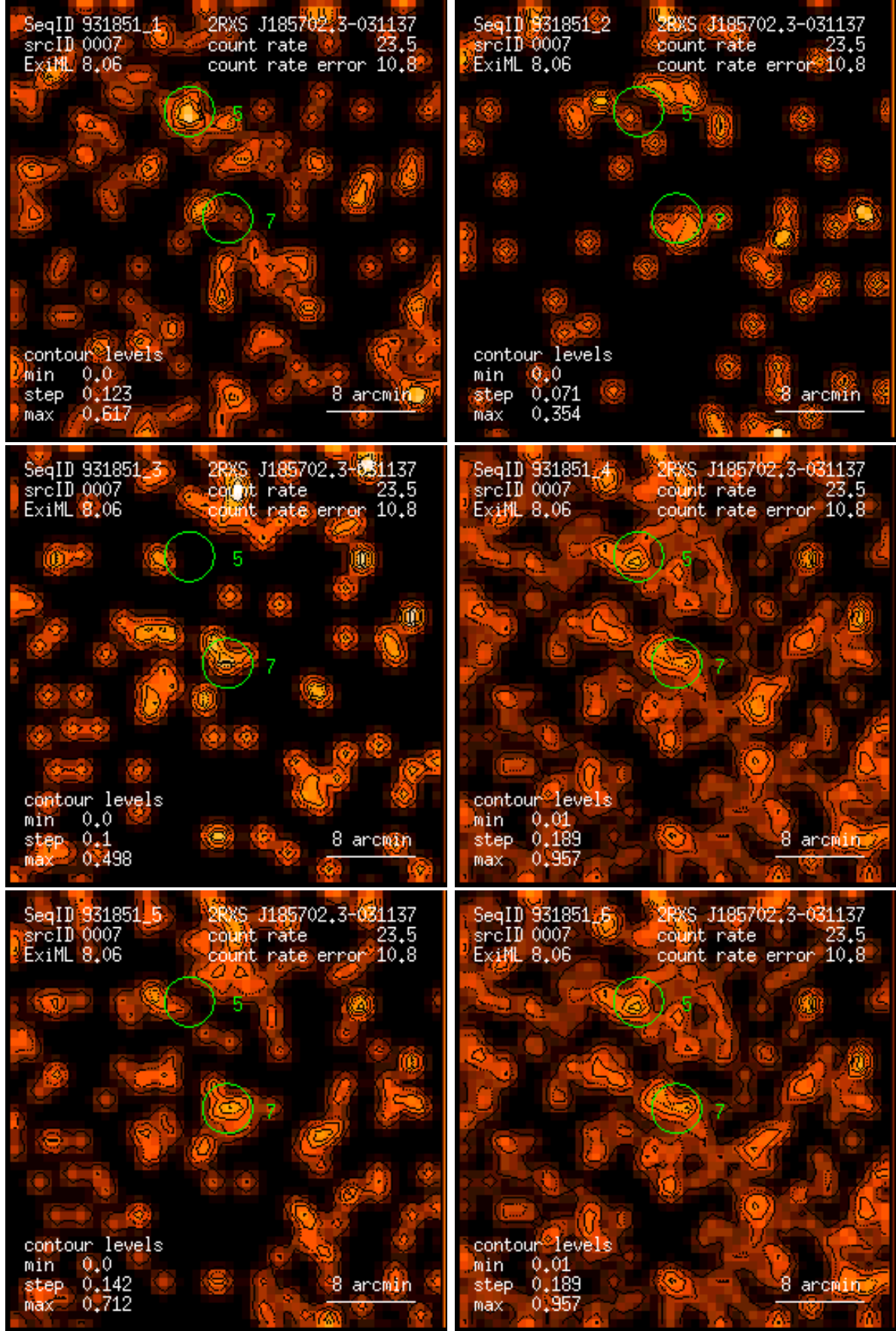
Figure 7: RASS 931851: detection 0007: band rate images, Gaussian filter: (1) PSPC channels 11 – 41, (2) 52 – 90, (3) 91 – 201, (4) 11 – 235, (5) 52 – 201, (6) 11 – 201. Broad band rates in counts/ks. Band rate contour levels in counts/ks/arcmin 2 .
