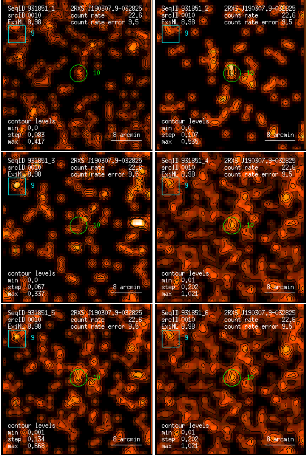
Figure 10: RASS 931851: detection 0010: band rate images, Gaussian filter: (1) PSPC channels 11 – 41, (2) 52 – 90, (3) 91 – 201, (4) 11 – 235, (5) 52 – 201, (6) 11 – 201. Broad band rates in counts/ks. Band rate contour levels in counts/ks/arcmin 2 .
