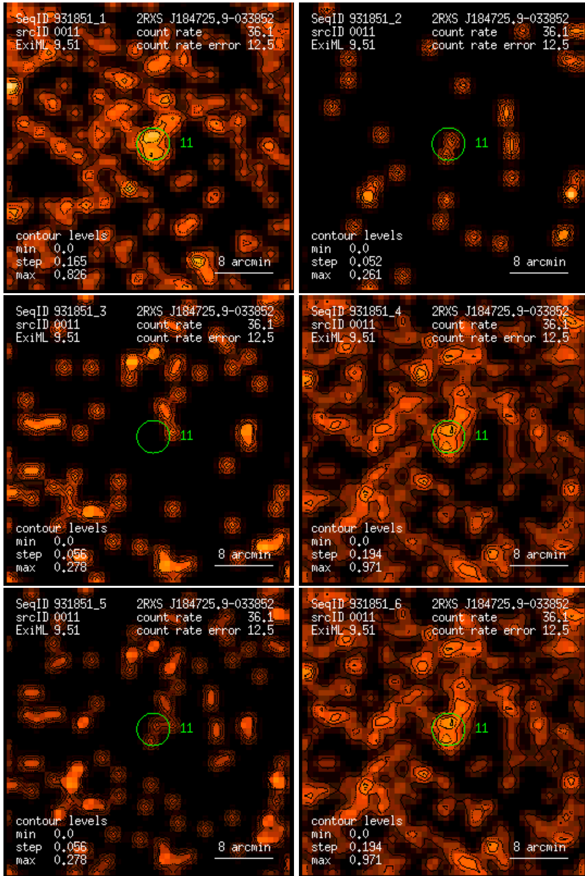
Figure 11: RASS 931851: detection 0011: band rate images, Gaussian filter: (1) PSPC channels 11 – 41, (2) 52 – 90, (3) 91 – 201, (4) 11 – 235, (5) 52 – 201, (6) 11 – 201. Broad band rates in counts/ks. Band rate contour levels in counts/ks/arcmin 2 .
