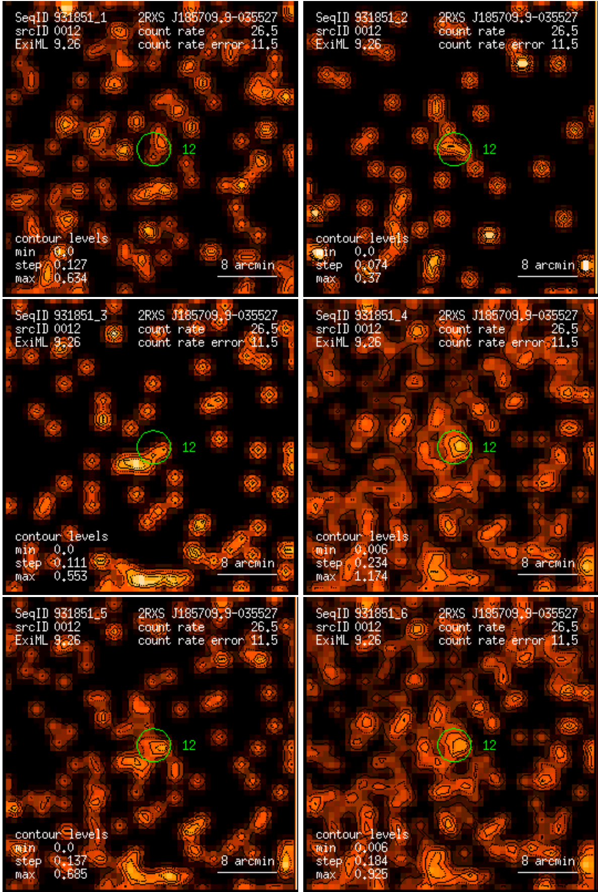
Figure 12: RASS 931851: detection 0012: band rate images, Gaussian filter: (1) PSPC channels 11 – 41, (2) 52 – 90, (3) 91 – 201, (4) 11 – 235, (5) 52 – 201, (6) 11 – 201. Broad band rates in counts/ks. Band rate contour levels in counts/ks/arcmin 2 .
