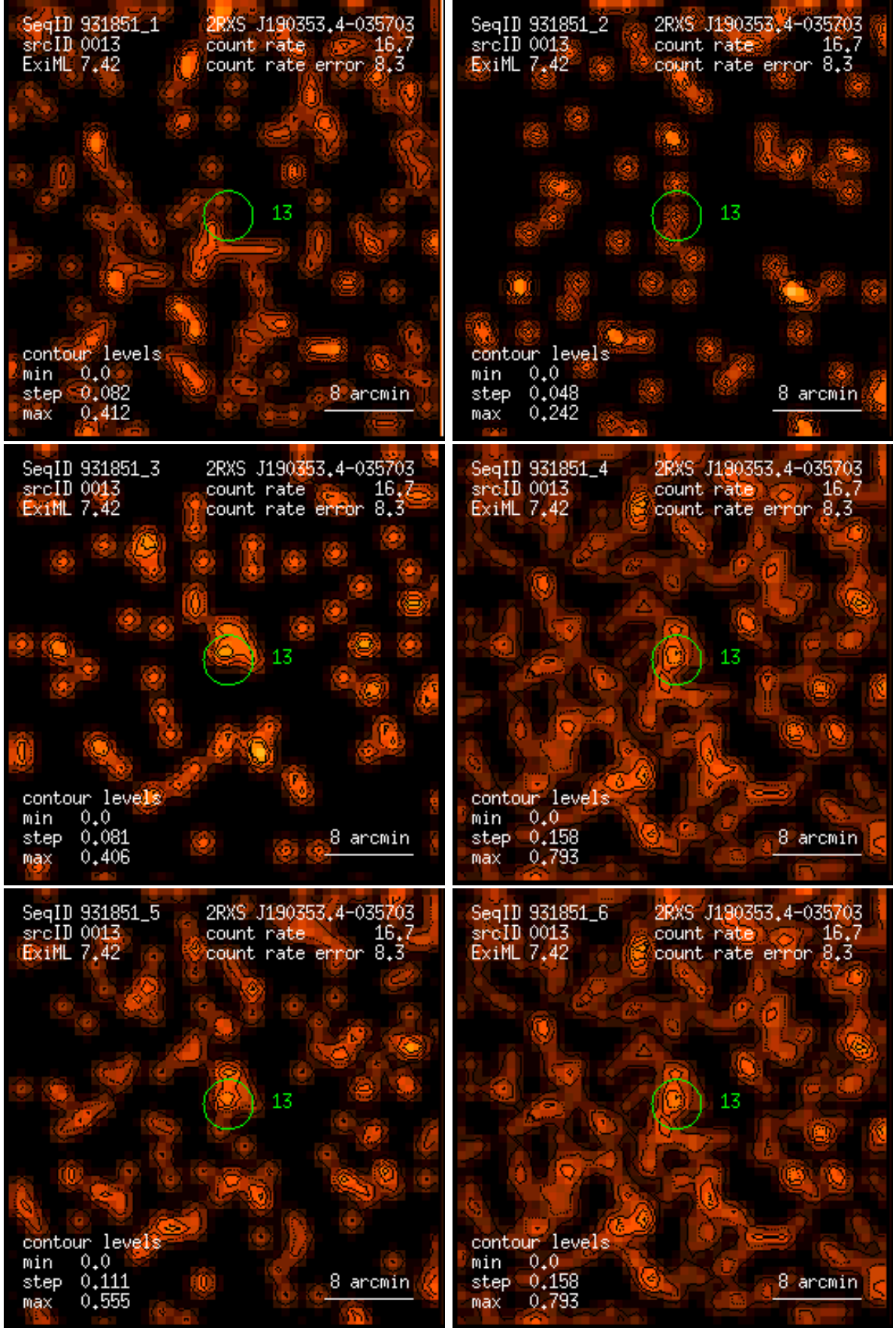
Figure 13: RASS 931851: detection 0013: band rate images, Gaussian filter: (1) PSPC channels 11 – 41, (2) 52 – 90, (3) 91 – 201, (4) 11 – 235, (5) 52 – 201, (6) 11 – 201. Broad band rates in counts/ks. Band rate contour levels in counts/ks/arcmin 2 .
