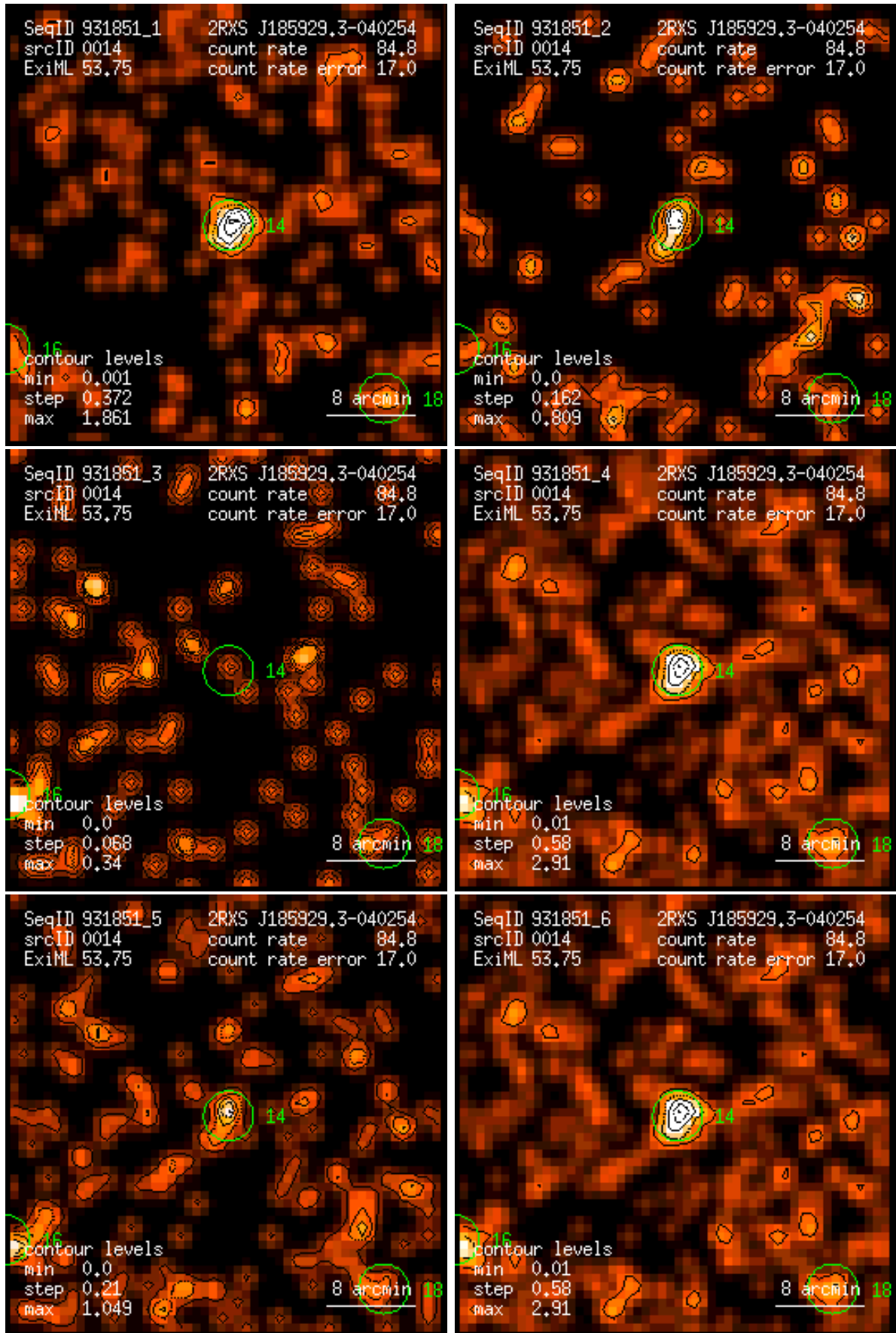
Figure 14: RASS 931851: detection 0014: band rate images, Gaussian filter: (1) PSPC channels 11 – 41, (2) 52 – 90, (3) 91 – 201, (4) 11 – 235, (5) 52 – 201, (6) 11 – 201. Broad band rates in counts/ks. Band rate contour levels in counts/ks/arcmin 2 .
