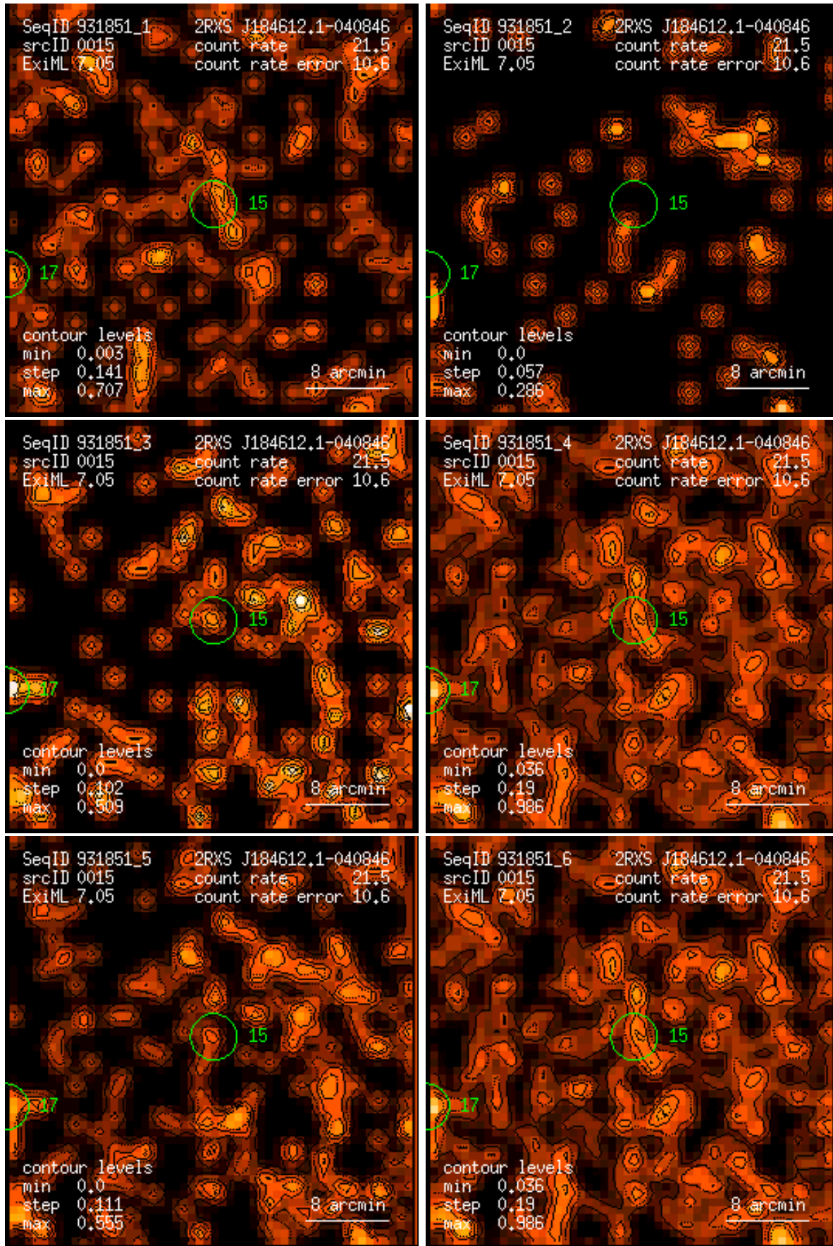
Figure 15: RASS 931851: detection 0015: band rate images, Gaussian filter: (1) PSPC channels 11 – 41, (2) 52 – 90, (3) 91 – 201, (4) 11 – 235, (5) 52 – 201, (6) 11 – 201. Broad band rates in counts/ks. Band rate contour levels in counts/ks/arcmin 2 .
