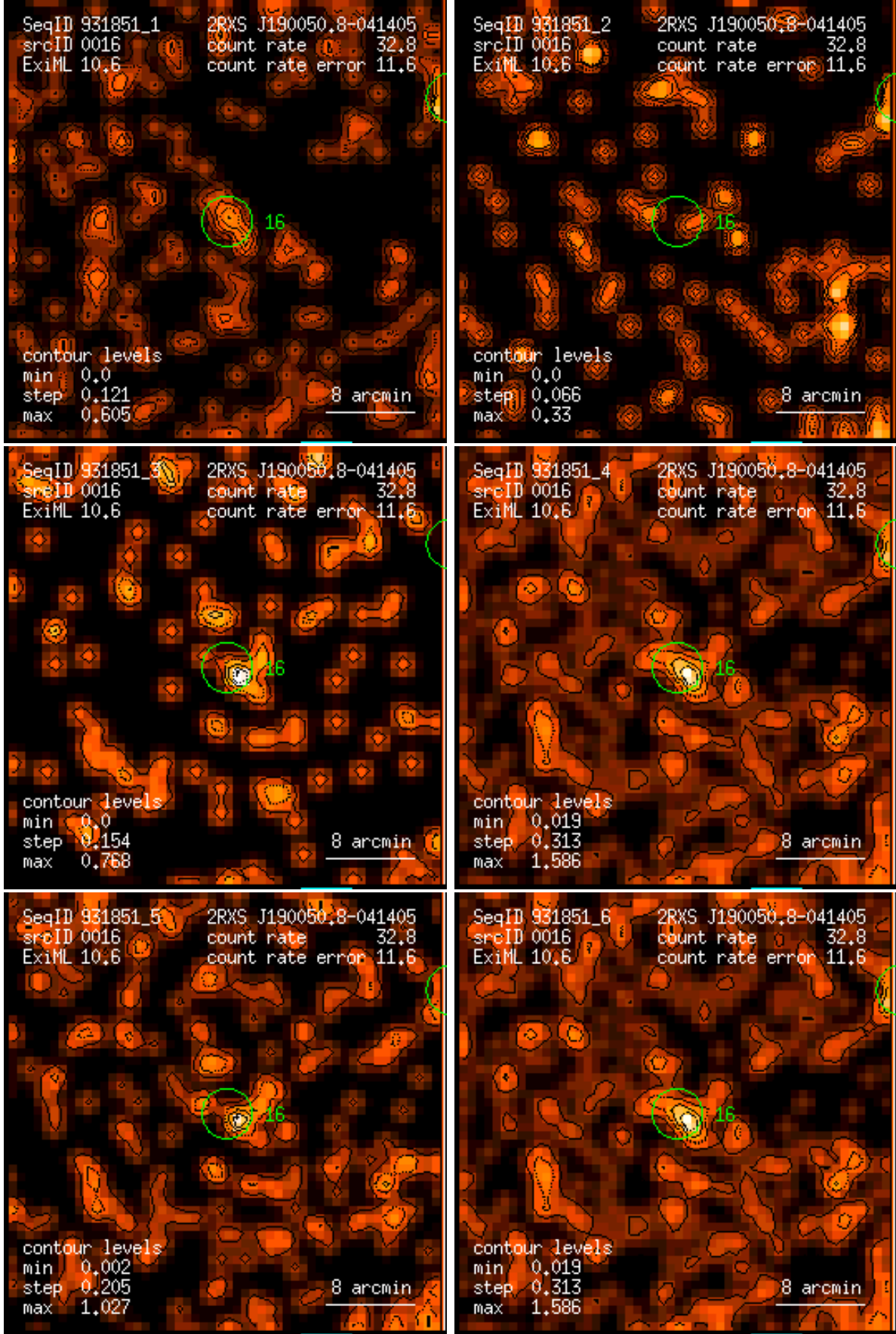
Figure 16: RASS 931851: detection 0016: band rate images, Gaussian filter: (1) PSPC channels 11 – 41, (2) 52 – 90, (3) 91 – 201, (4) 11 – 235, (5) 52 – 201, (6) 11 – 201. Broad band rates in counts/ks. Band rate contour levels in counts/ks/arcmin 2 .
