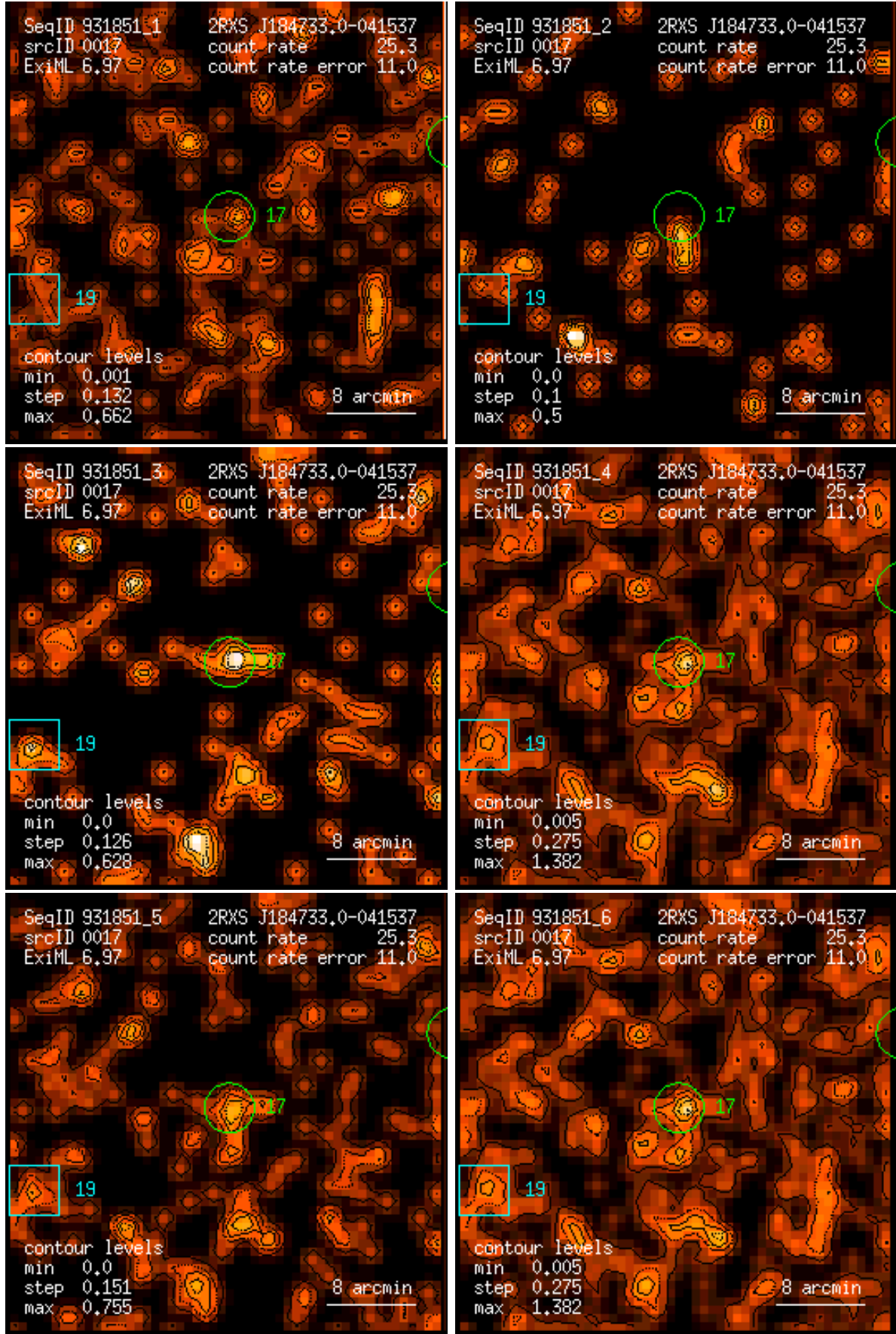
Figure 17: RASS 931851: detection 0017: band rate images, Gaussian filter: (1) PSPC channels 11 – 41, (2) 52 – 90, (3) 91 – 201, (4) 11 – 235, (5) 52 – 201, (6) 11 – 201. Broad band rates in counts/ks. Band rate contour levels in counts/ks/arcmin 2 .
