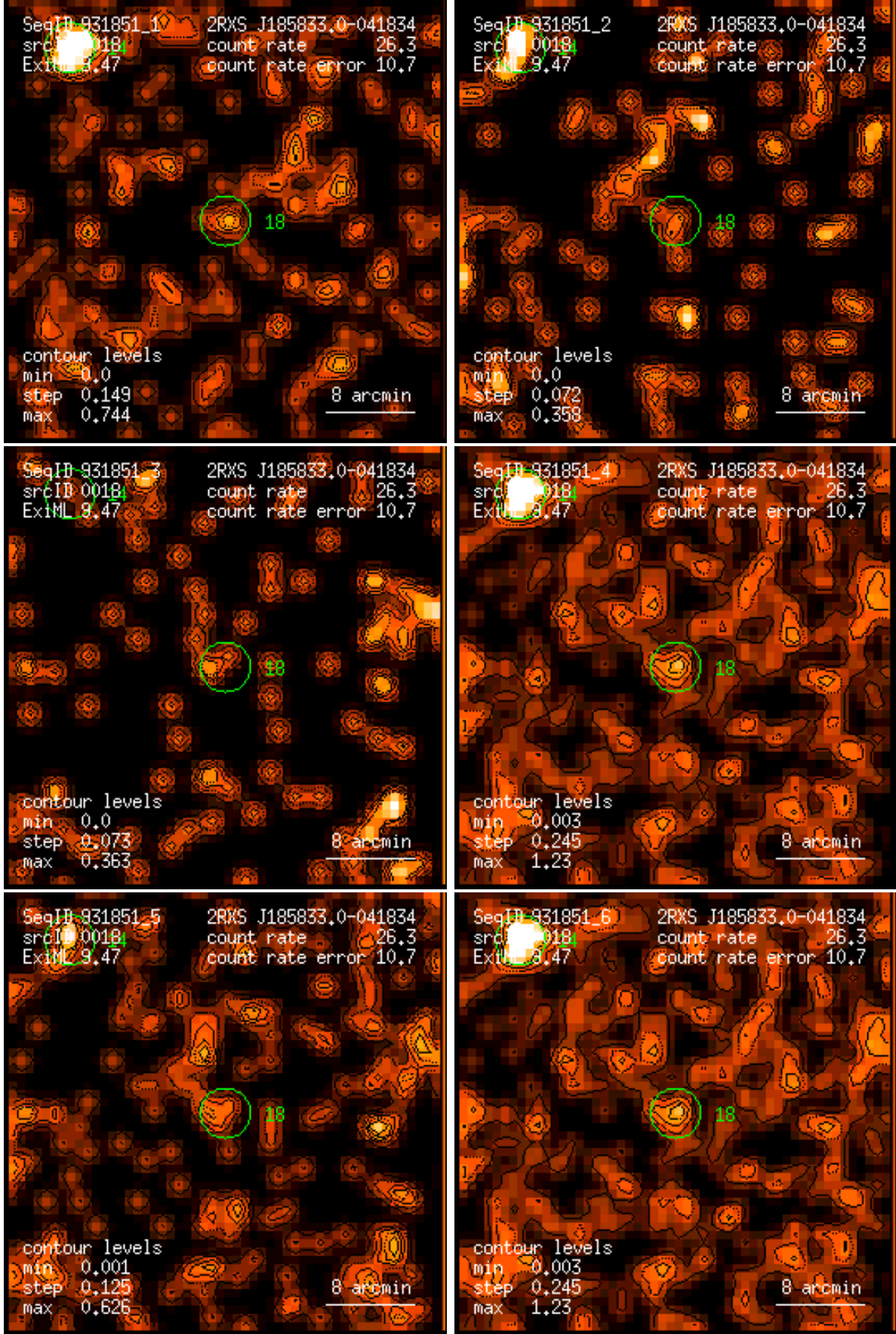
Figure 18: RASS 931851: detection 0018: band rate images, Gaussian filter: (1) PSPC channels 11 – 41, (2) 52 – 90, (3) 91 – 201, (4) 11 – 235, (5) 52 – 201, (6) 11 – 201. Broad band rates in counts/ks. Band rate contour levels in counts/ks/arcmin 2 .
