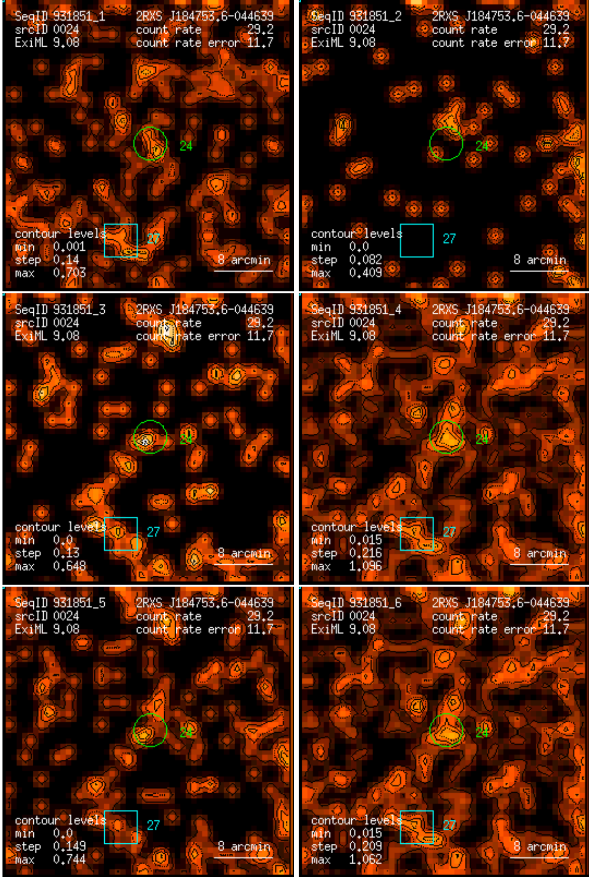
Figure 24: RASS 931851: detection 0024: band rate images, Gaussian filter: (1) PSPC channels 11 – 41, (2) 52 – 90, (3) 91 – 201, (4) 11 – 235, (5) 52 – 201, (6) 11 – 201. Broad band rates in counts/ks. Band rate contour levels in counts/ks/arcmin 2 .
