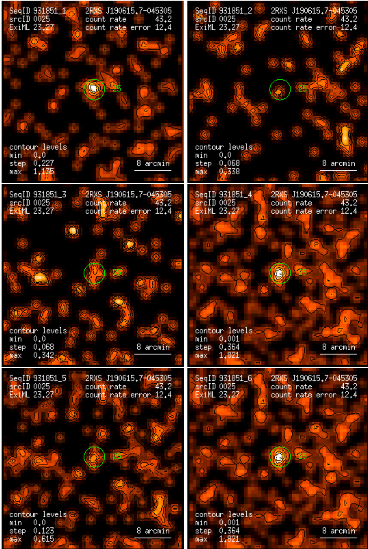
Figure 25: RASS 931851: detection 0025: band rate images, Gaussian filter: (1) PSPC channels 11 – 41, (2) 52 – 90, (3) 91 – 201, (4) 11 – 235, (5) 52 – 201, (6) 11 – 201. Broad band rates in counts/ks. Band rate contour levels in counts/ks/arcmin 2 .
