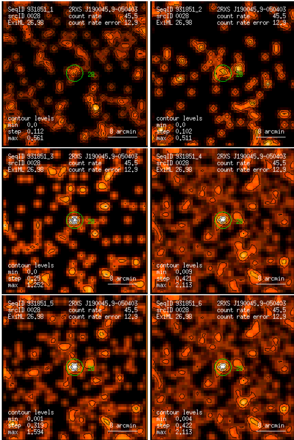
Figure 28: RASS 931851: detection 0028: band rate images, Gaussian filter: (1) PSPC channels 11 – 41, (2) 52 – 90, (3) 91 – 201, (4) 11 – 235, (5) 52 – 201, (6) 11 – 201. Broad band rates in counts/ks. Band rate contour levels in counts/ks/arcmin 2 .
