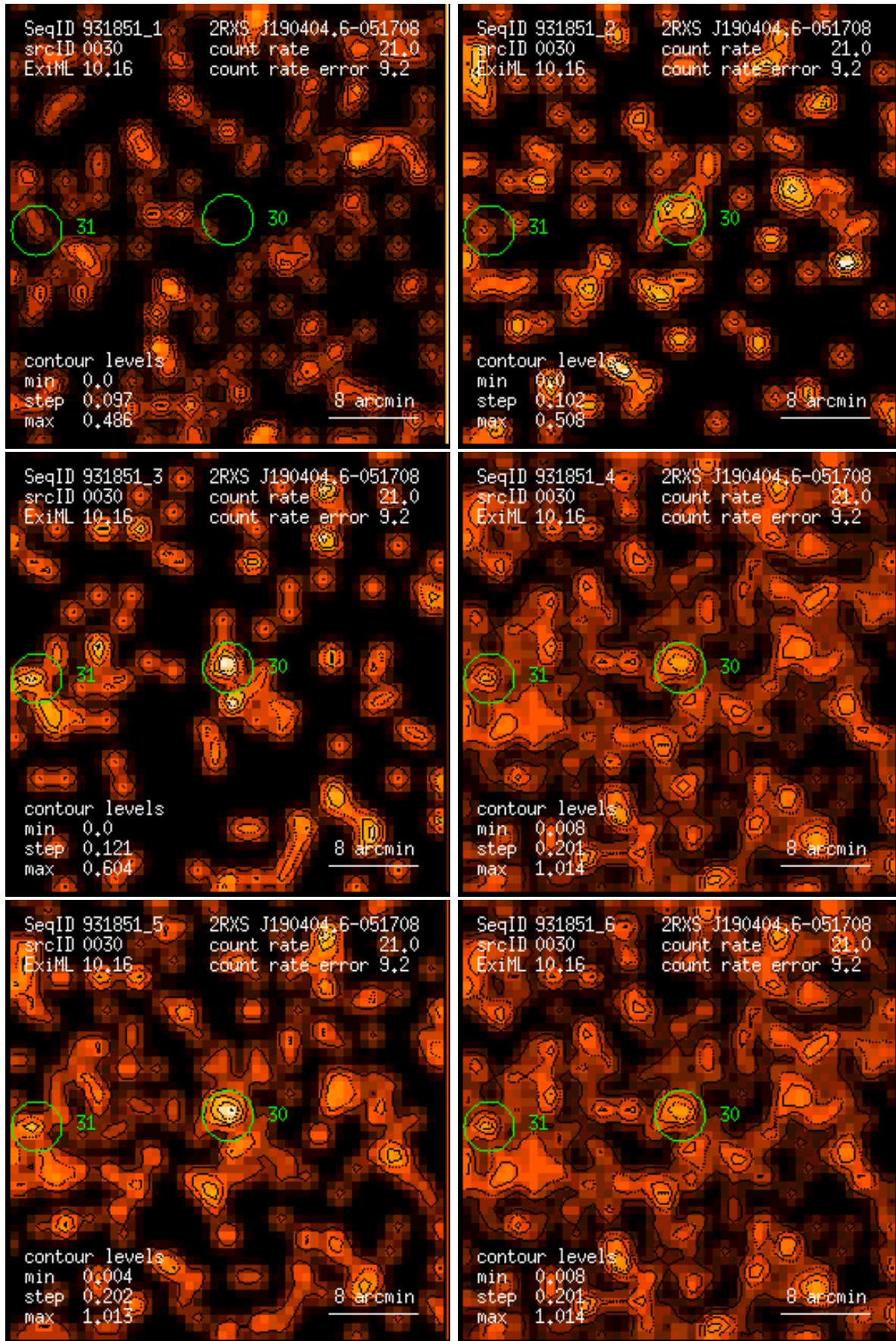
Figure 30: RASS 931851: detection 0030: band rate images, Gaussian filter: (1) PSPC channels 11 – 41, (2) 52 – 90, (3) 91 – 201, (4) 11 – 235, (5) 52 – 201, (6) 11 – 201. Broad band rates in counts/ks. Band rate contour levels in counts/ks/arcmin 2 .
