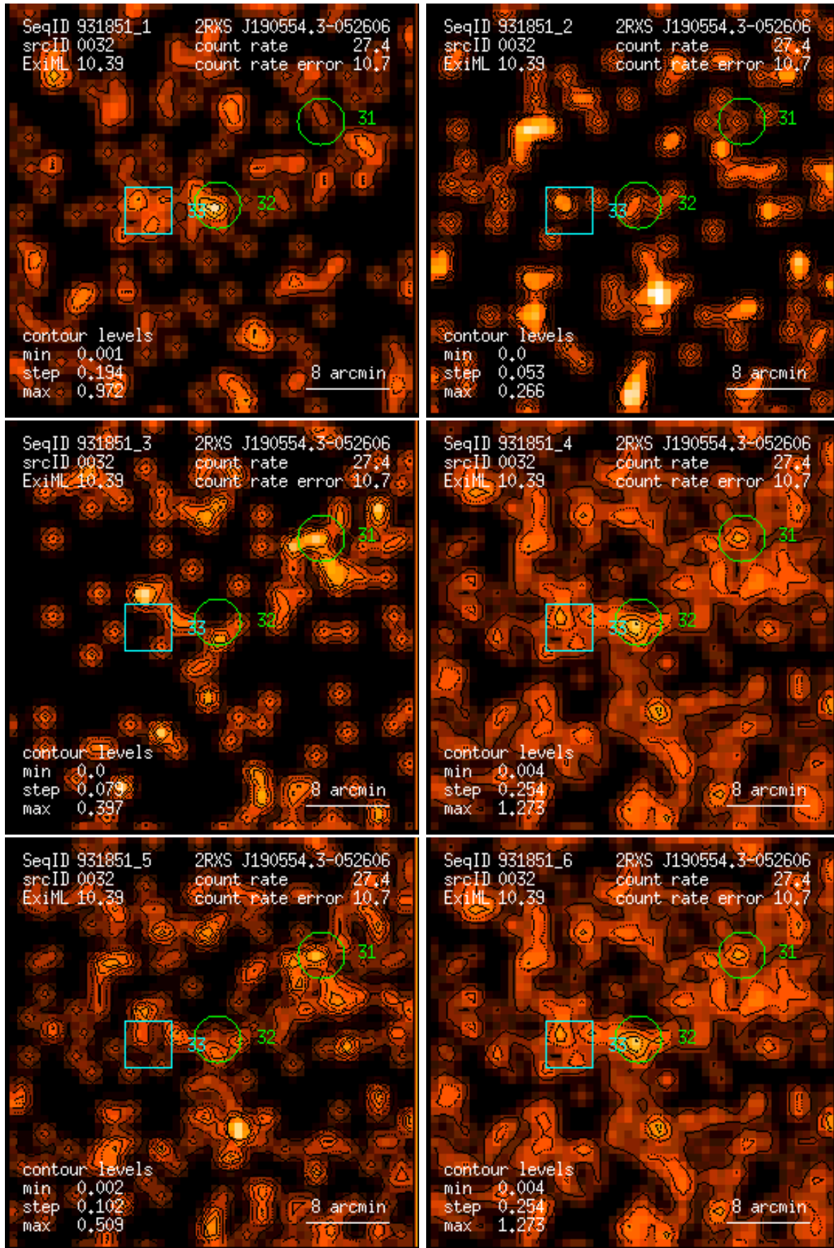
Figure 32: RASS 931851: detection 0032: band rate images, Gaussian filter: (1) PSPC channels 11 – 41, (2) 52 – 90, (3) 91 – 201, (4) 11 – 235, (5) 52 – 201, (6) 11 – 201. Broad band rates in counts/ks. Band rate contour levels in counts/ks/arcmin 2 .
