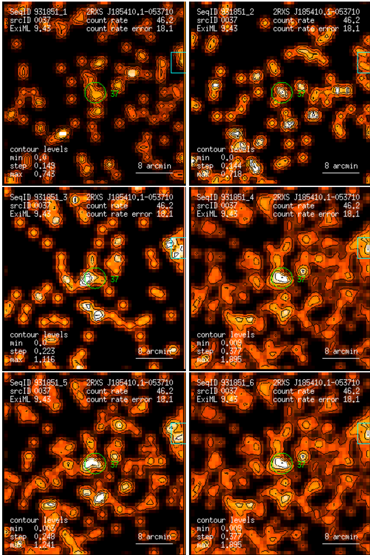
Figure 37: RASS 931851: detection 0037: band rate images, Gaussian filter: (1) PSPC channels 11 – 41, (2) 52 – 90, (3) 91 – 201, (4) 11 – 235, (5) 52 – 201, (6) 11 – 201. Broad band rates in counts/ks. Band rate contour levels in counts/ks/arcmin 2 .
