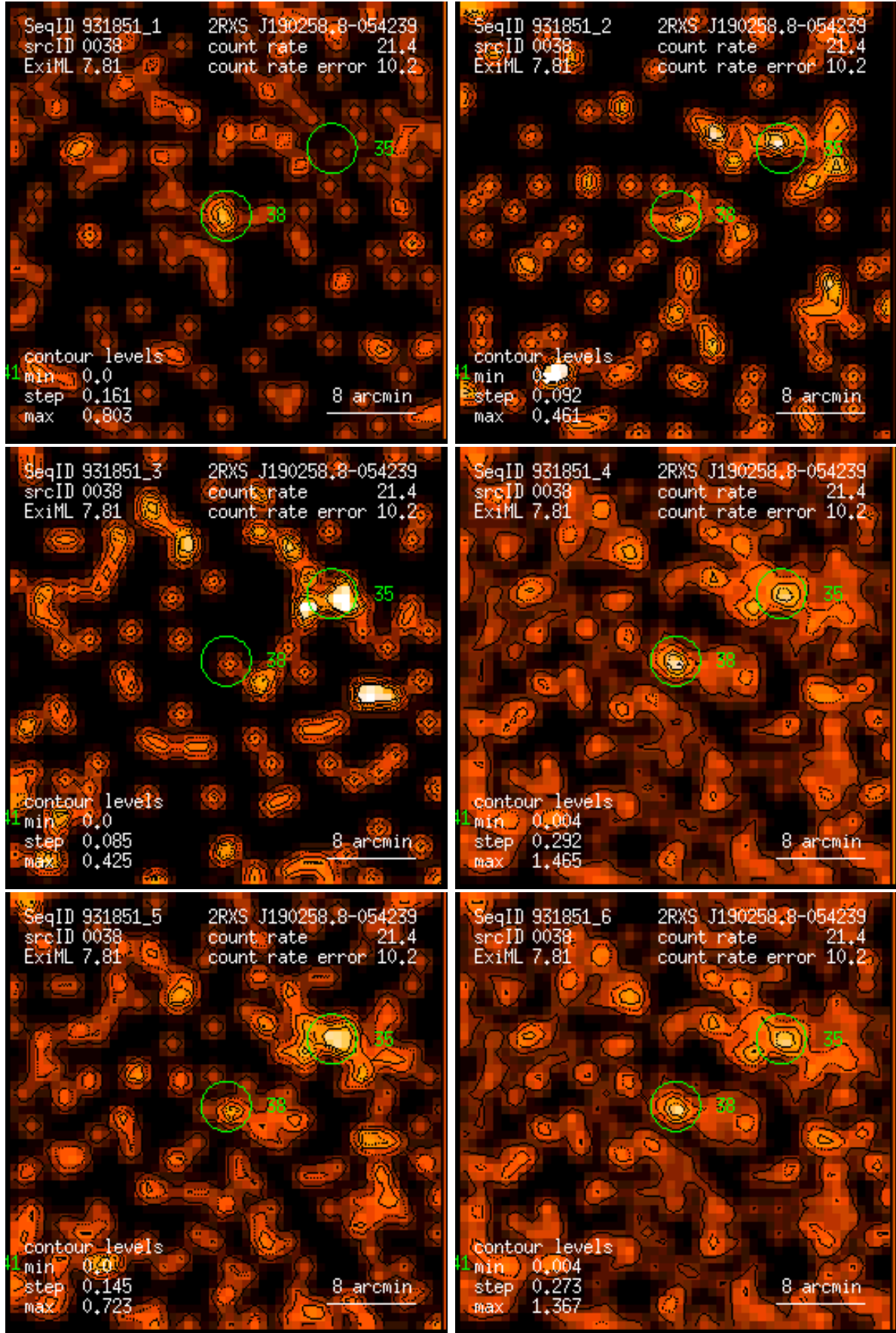
Figure 38: RASS 931851: detection 0038: band rate images, Gaussian filter: (1) PSPC channels 11 – 41, (2) 52 – 90, (3) 91 – 201, (4) 11 – 235, (5) 52 – 201, (6) 11 – 201. Broad band rates in counts/ks. Band rate contour levels in counts/ks/arcmin 2 .
